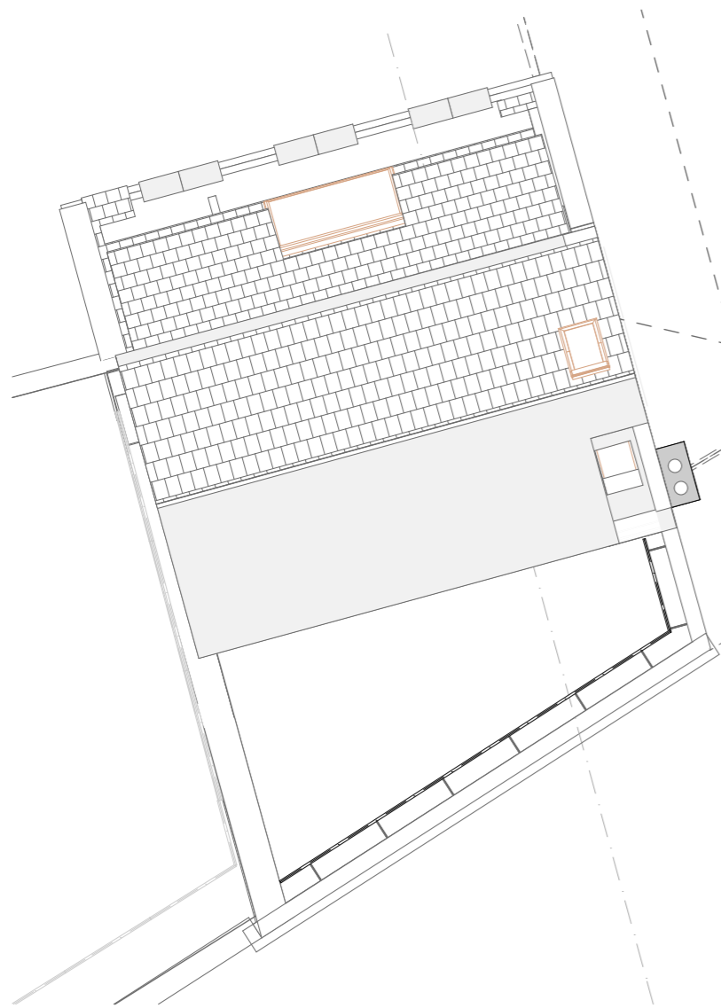
RF-Proposed Roof Plan 1:100
