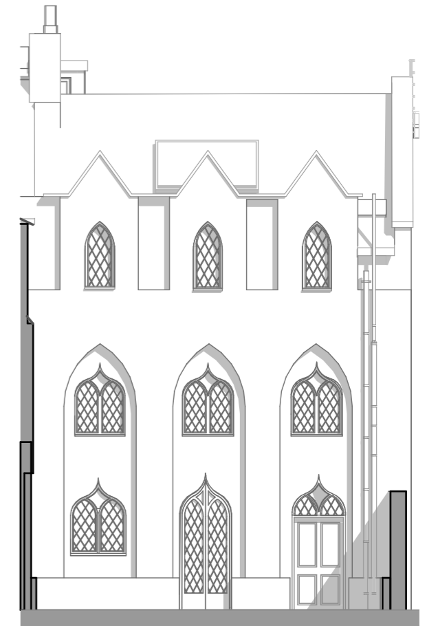
E-02 Rear Elevation 1:100
