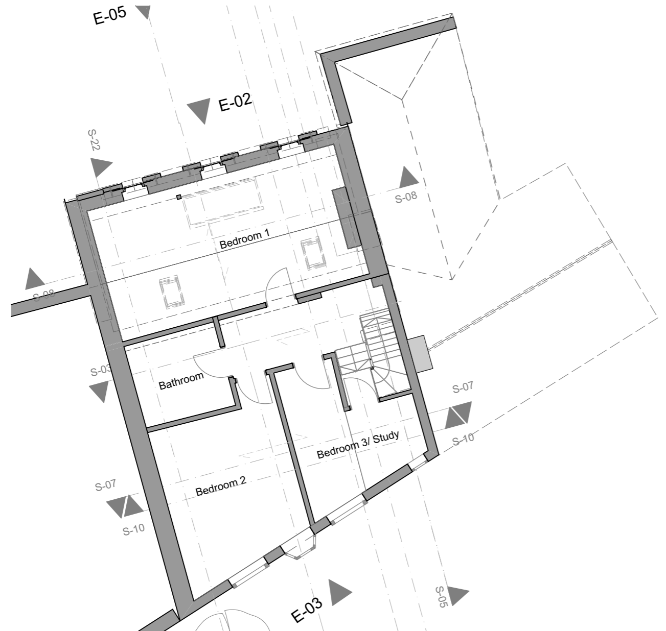
2. 02-Existing 2Fl 1:100
