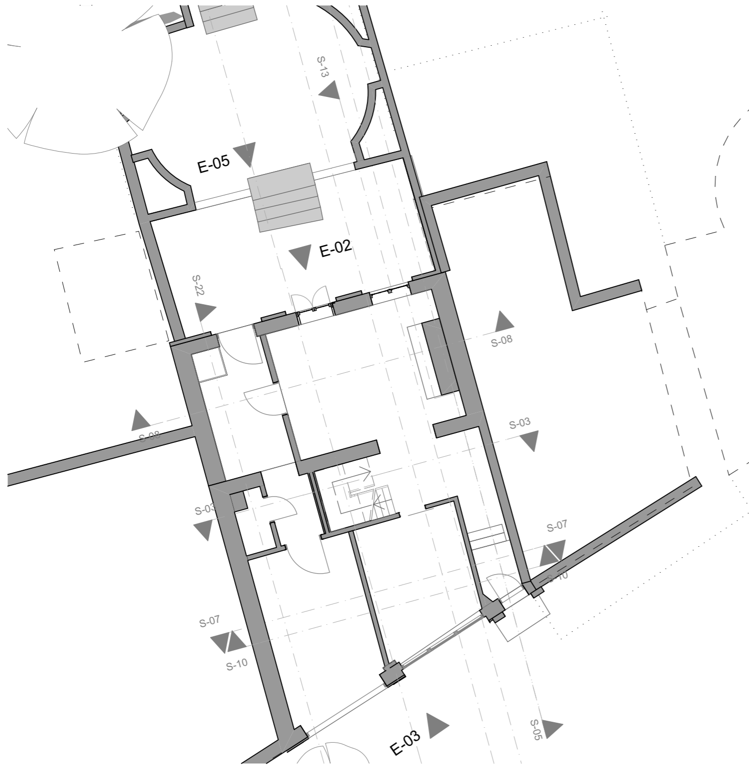
0. GF-Existing GF
