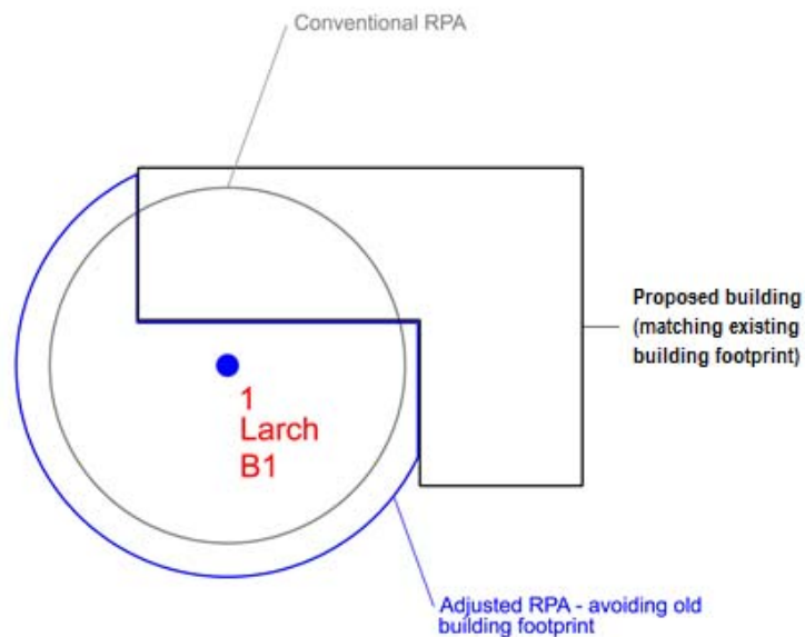
Figure 2 – Generic BS 5837 RPA Adjustments
