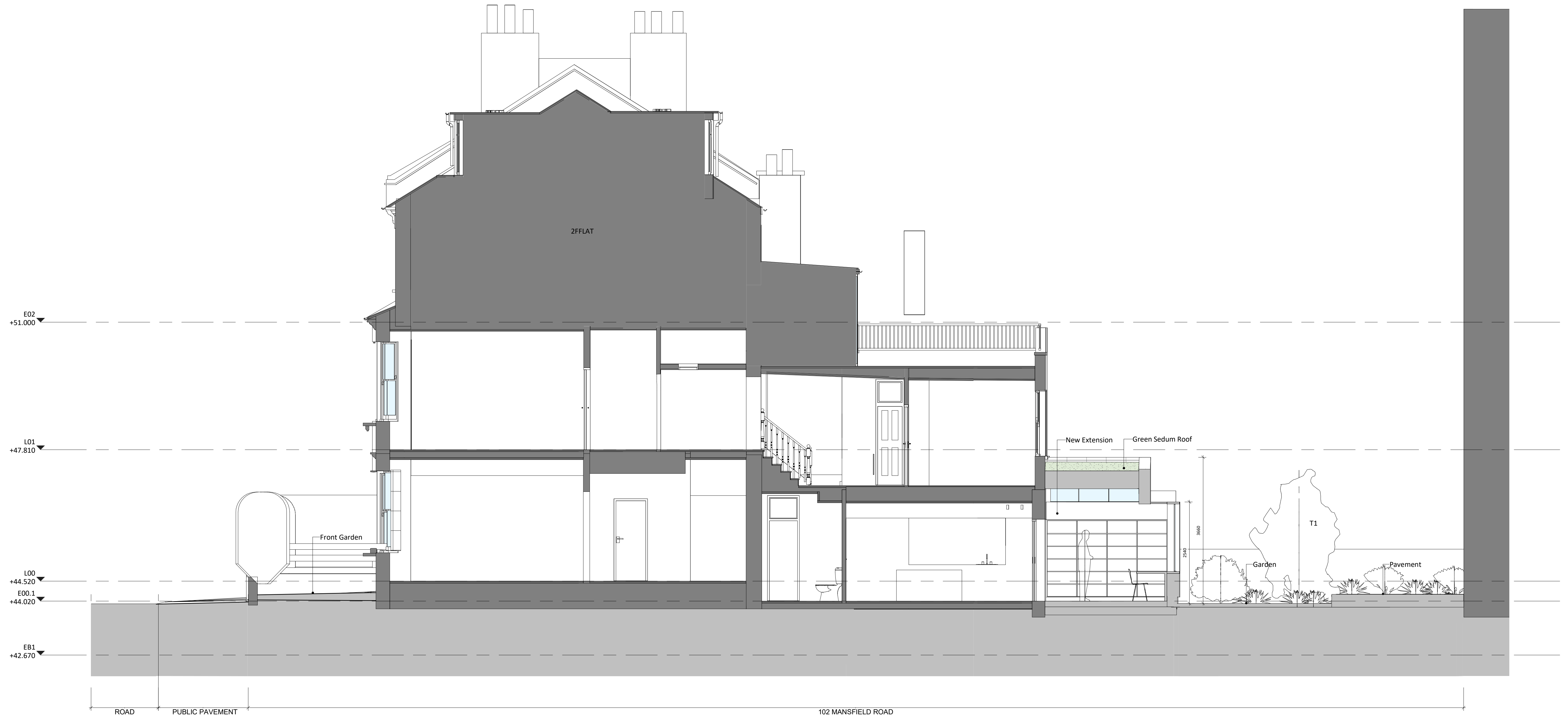
1 Section A 1:50
