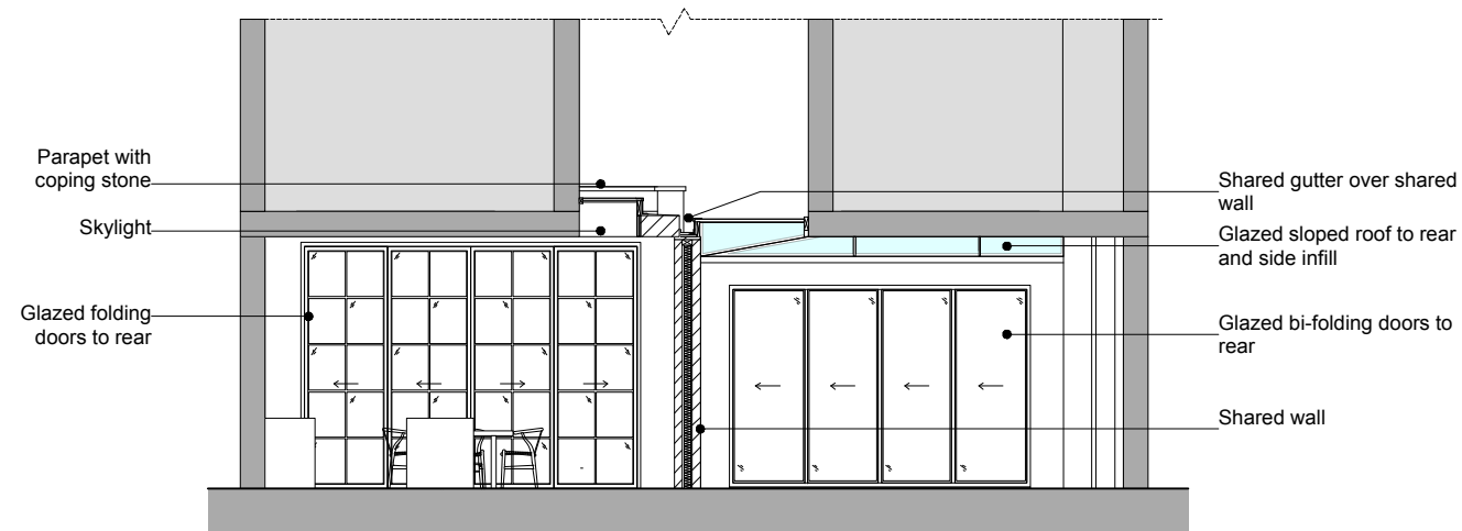
SECTION CC
