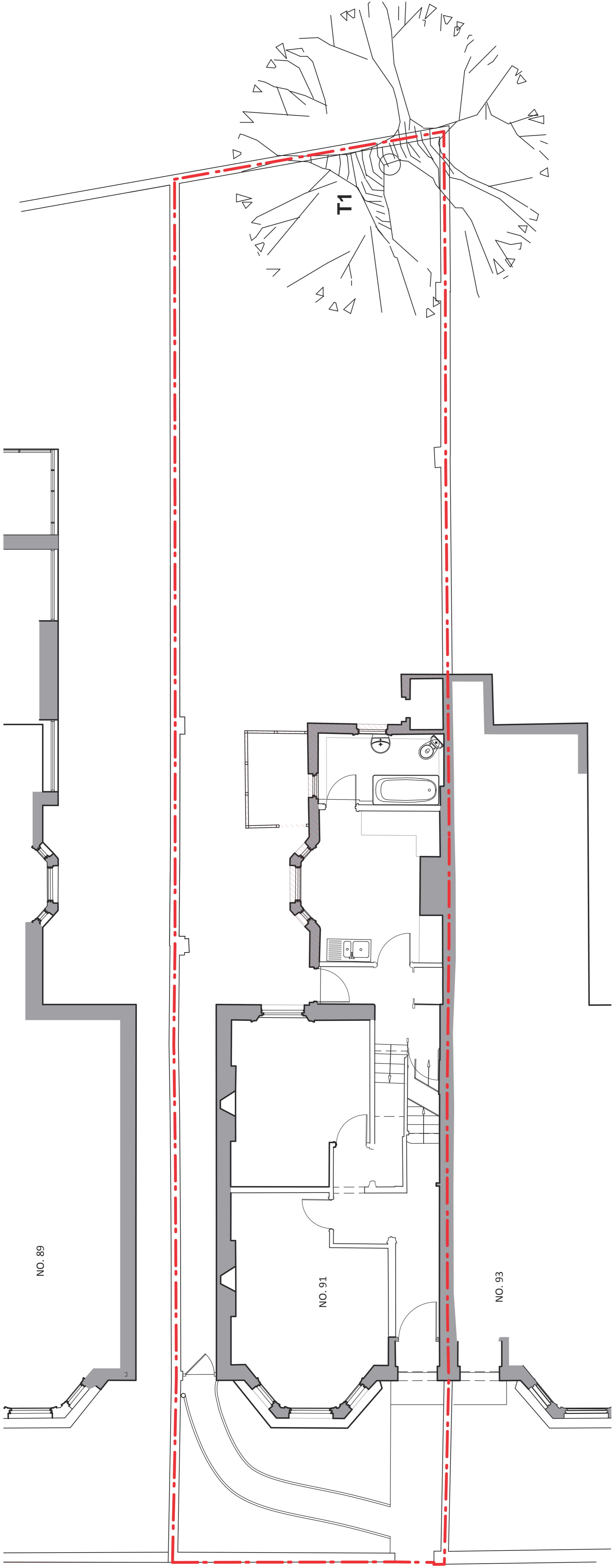
EXISTING GROUND FLOOR 1:100@ A3
