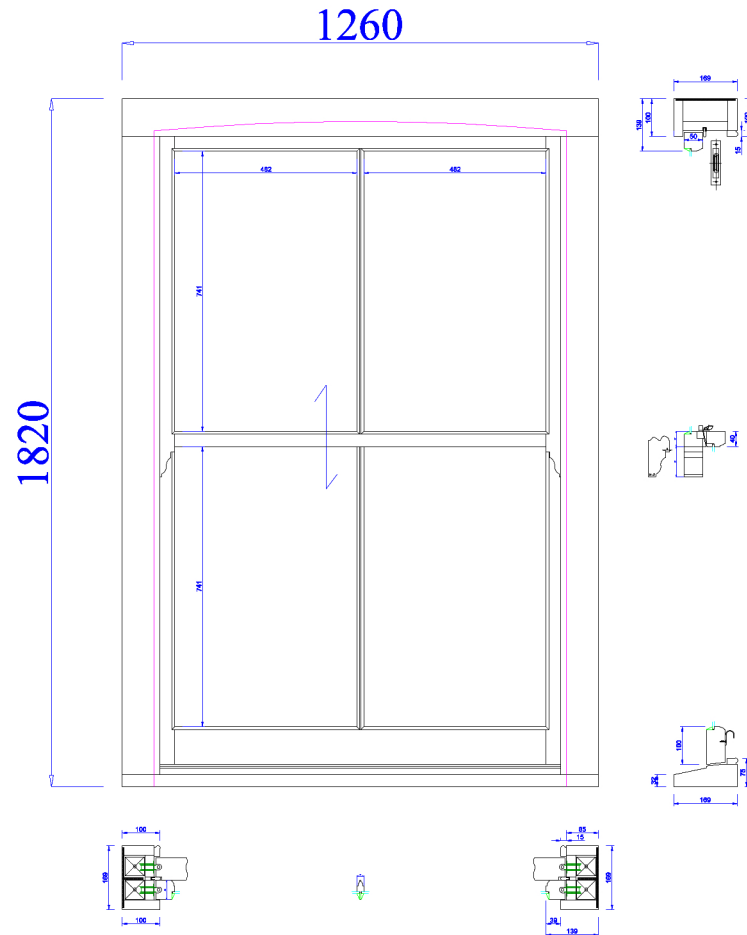
Existing Weighted Box Sash Window
