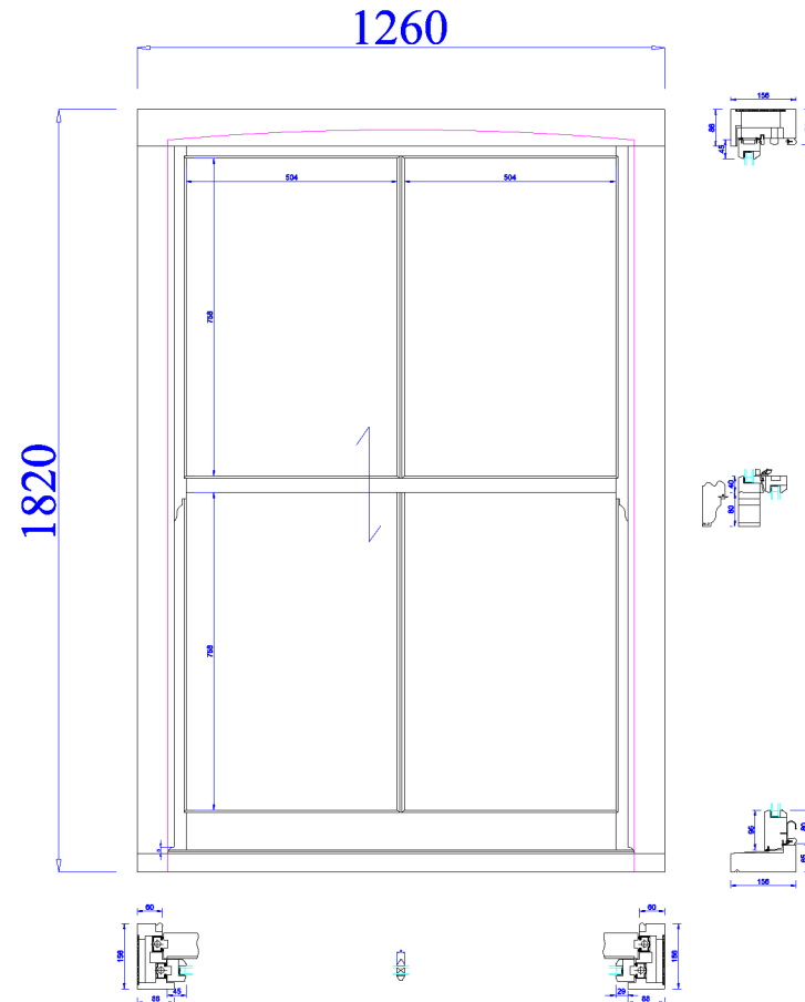
Proposed Sliding Sash
