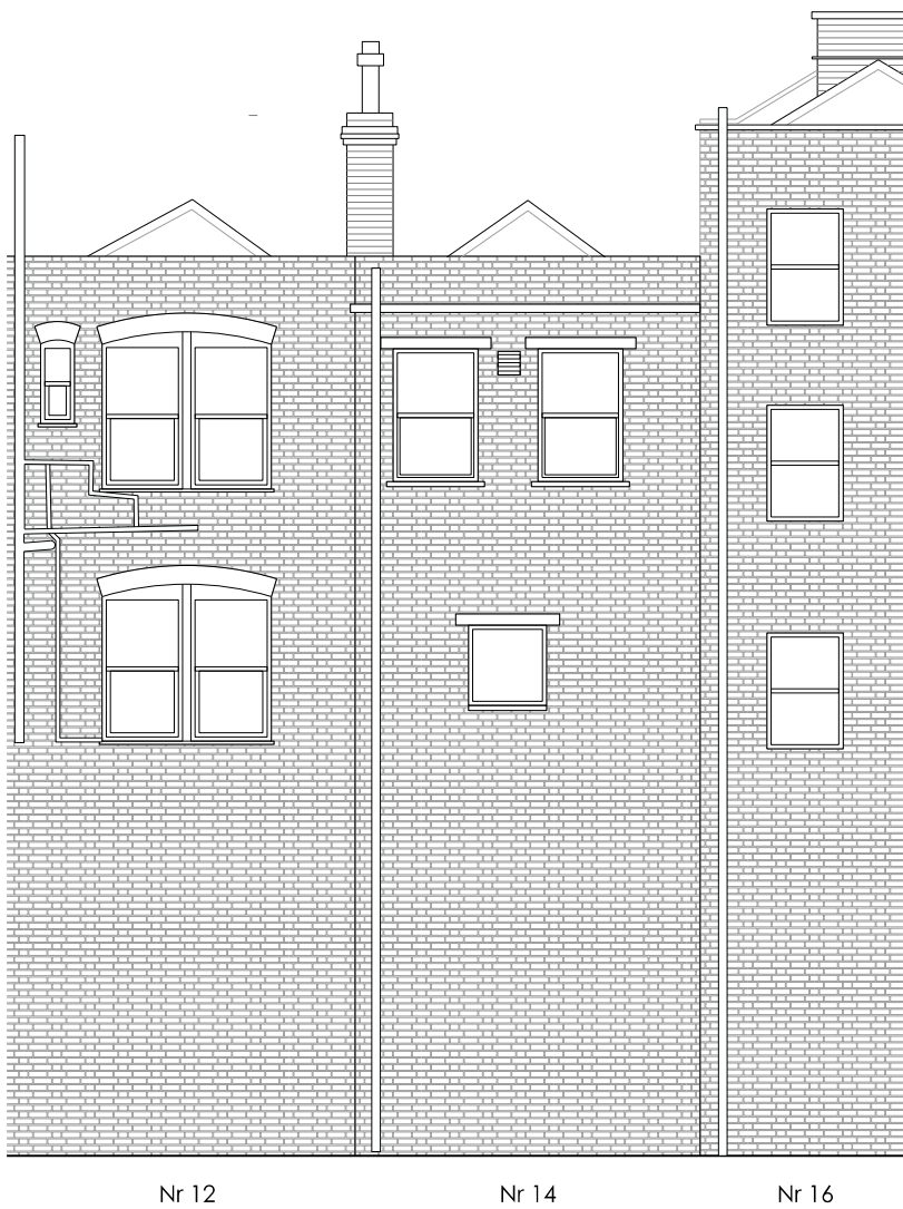
Existing north elevation
