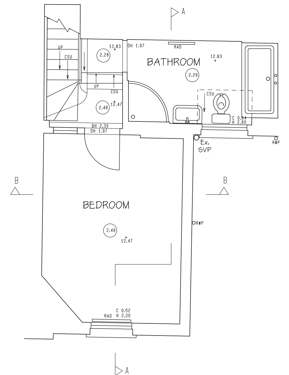
EXISTING FIRST FLOOR LAYOUT
