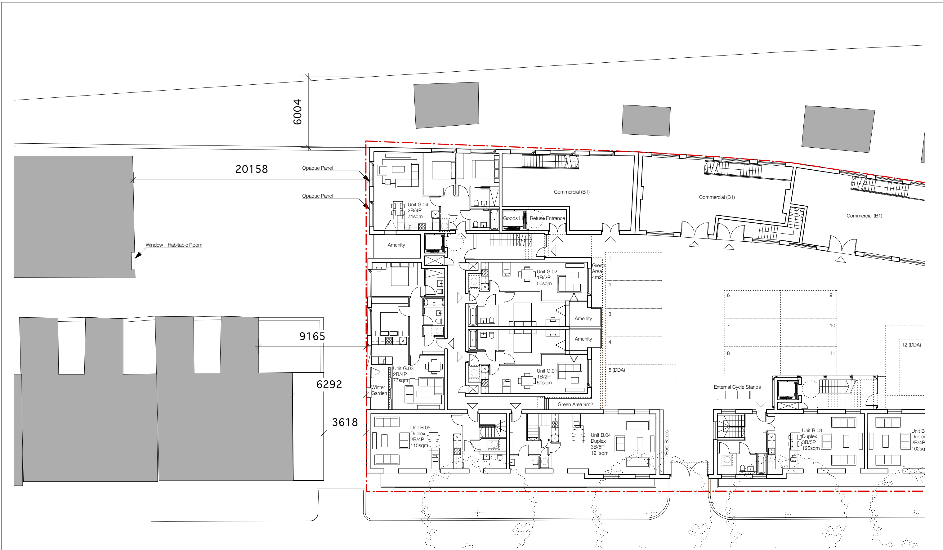
A Proposed Ground Floor General arrangement GA.20 1:100 @A1 1:200 @A3
