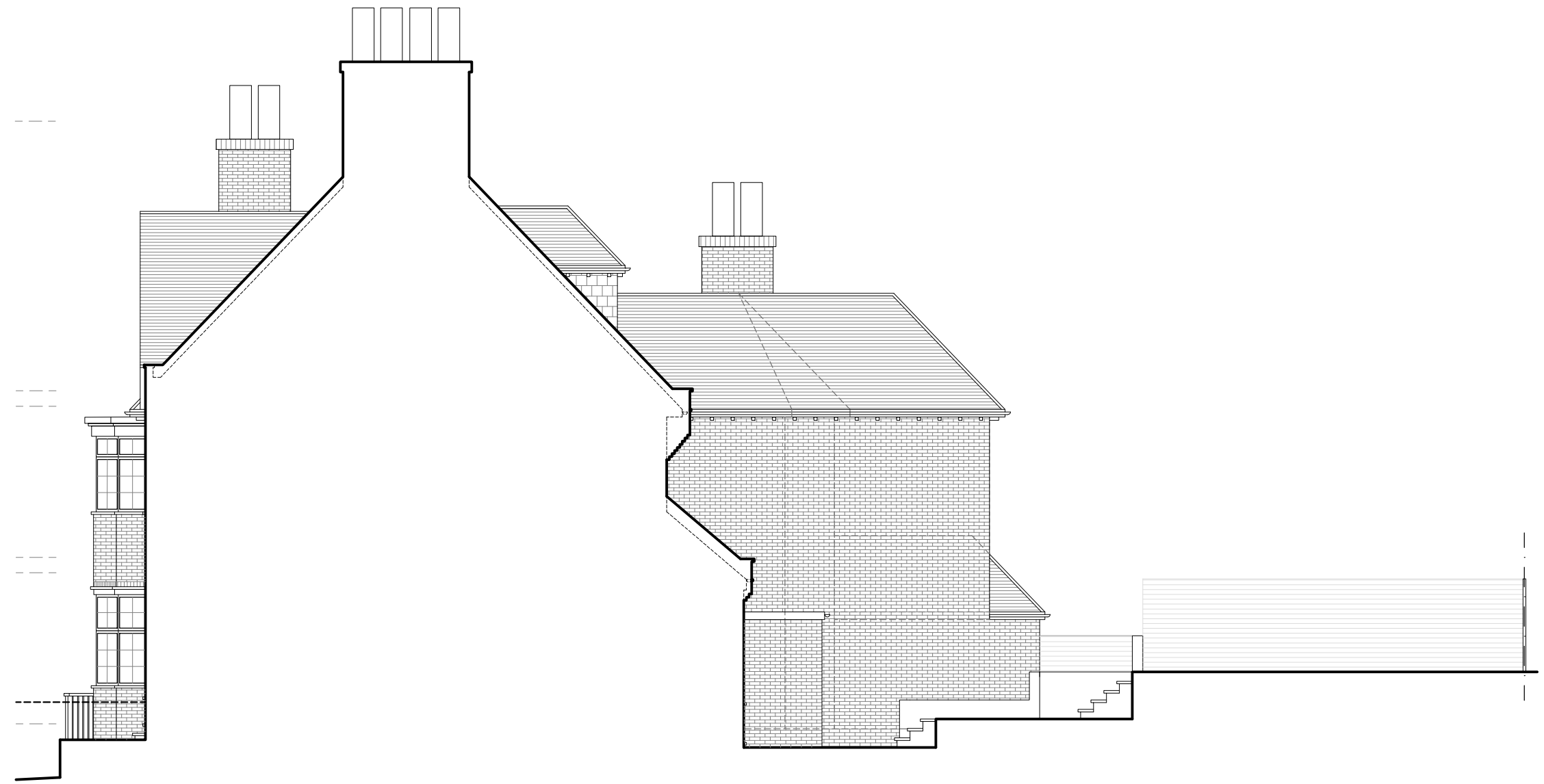
PROPOSED NORTH SIDE ELEVATION
