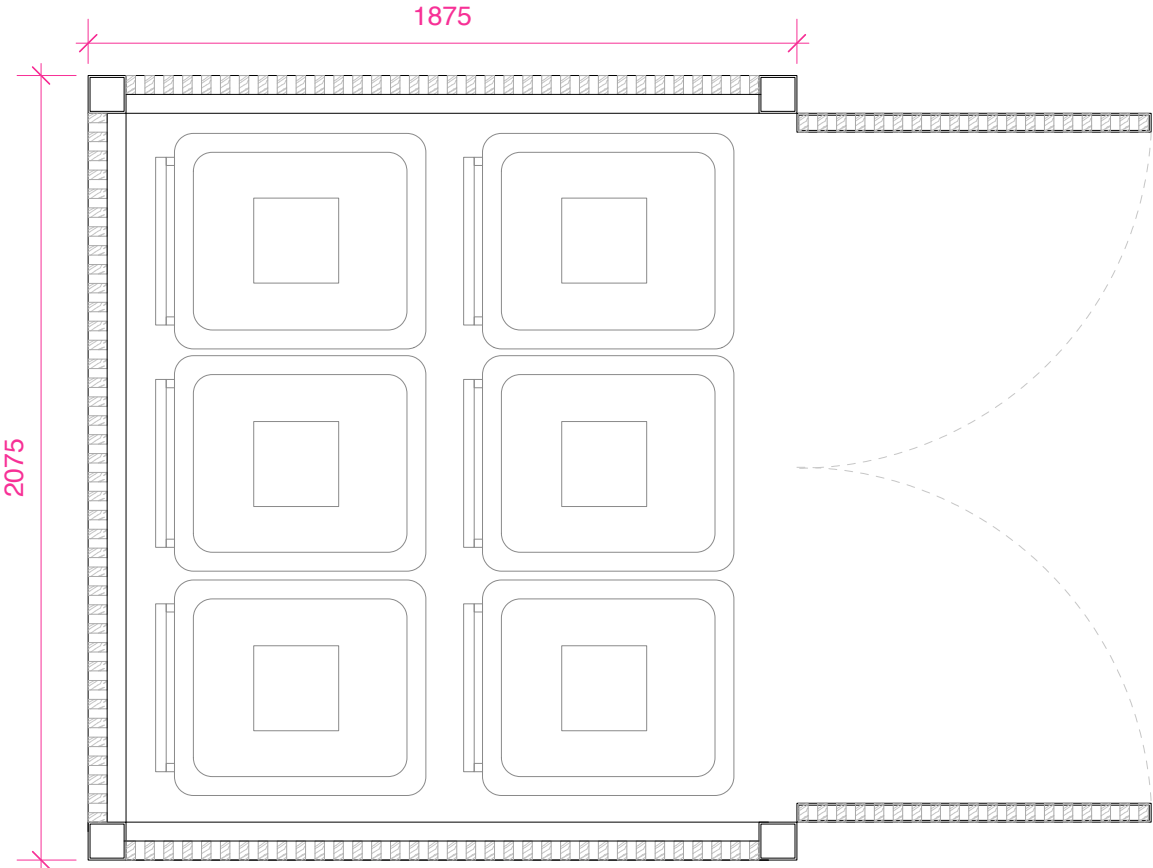
Proposed Bin Store Plan 1:20 @A3
