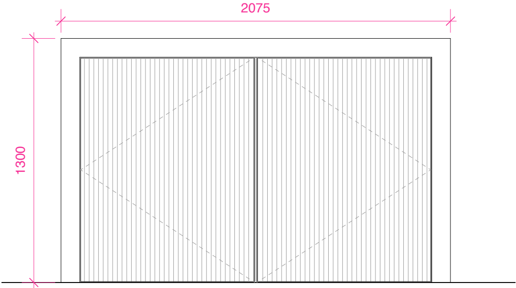
Proposed Front Elevation 1:20 @A3
