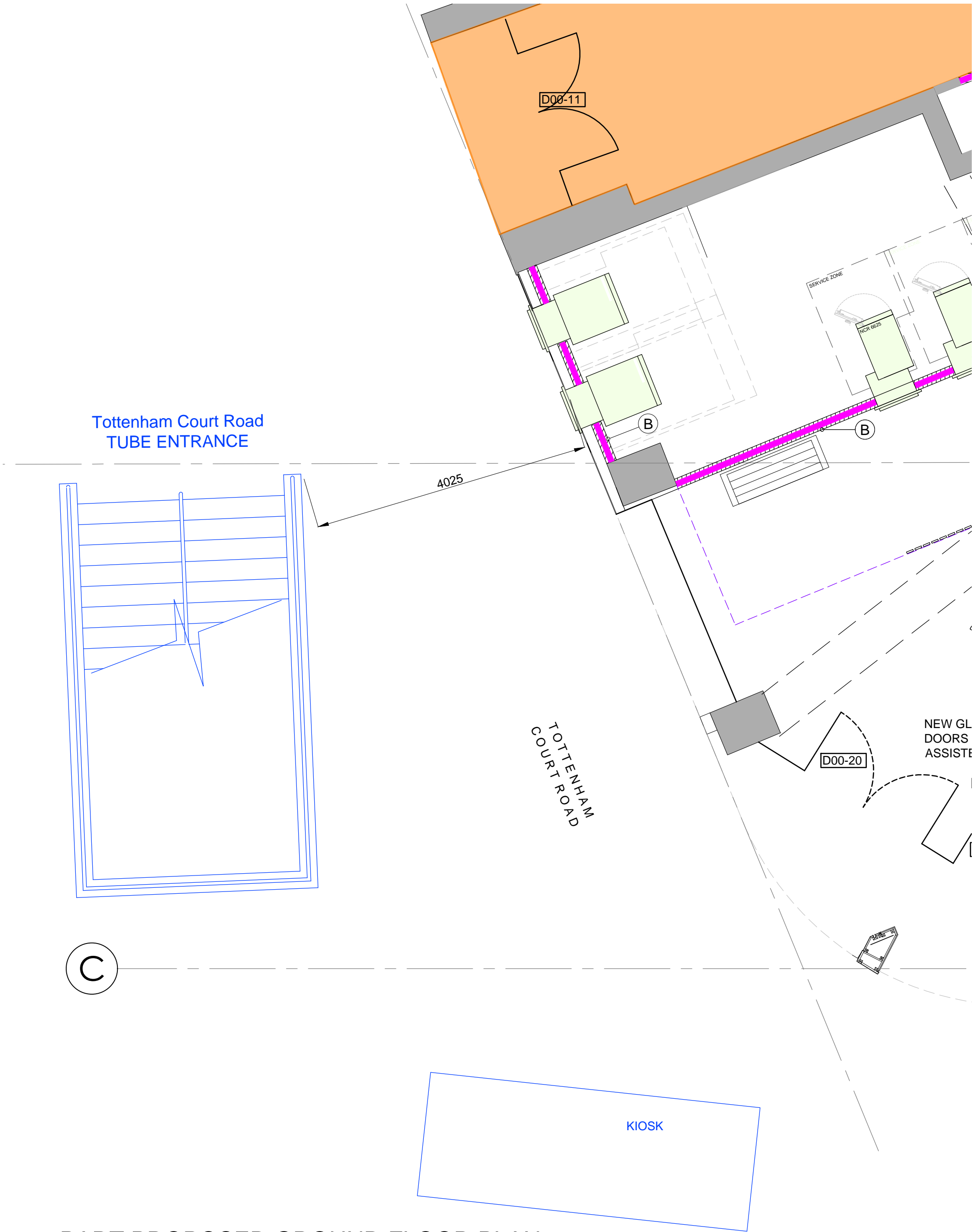
PART PROPOSED GROUND FLOOR PLAN TUBE ENTRANCE 50941725-AR01-00-SK01 Scale 1:50
