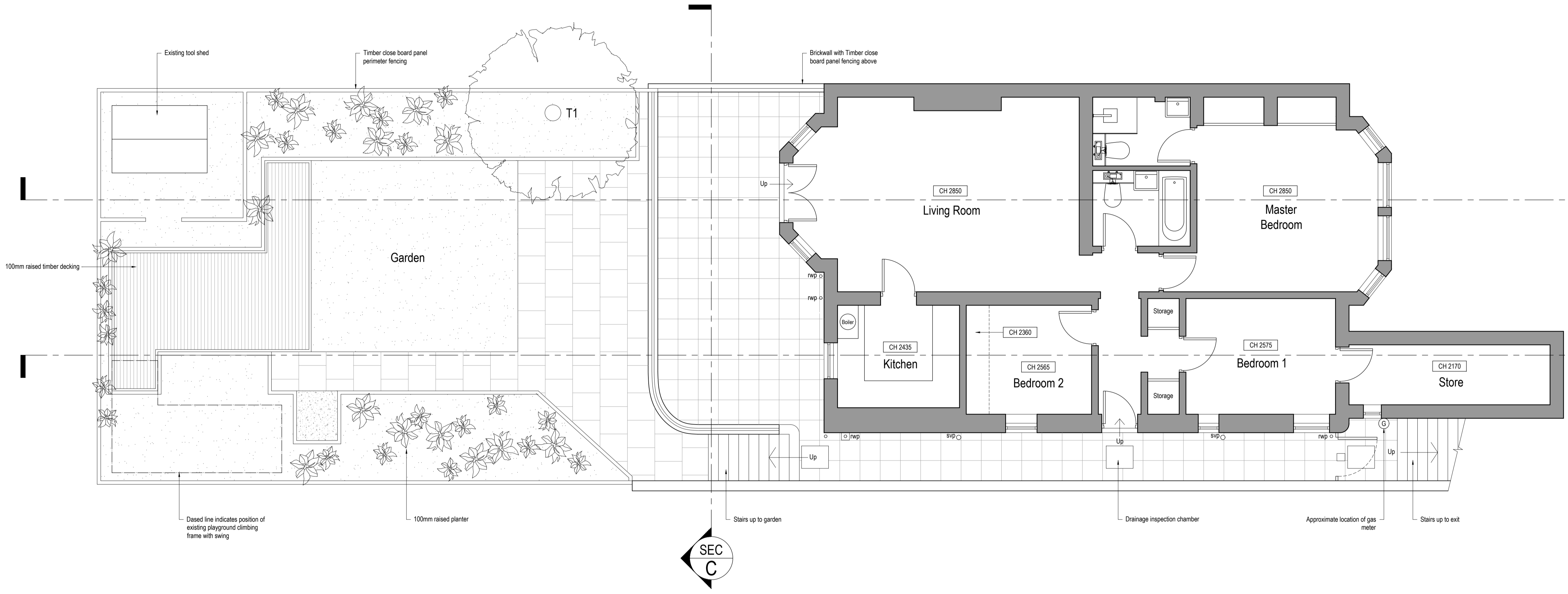
Existing Ground Floor General Arrangement Plan
