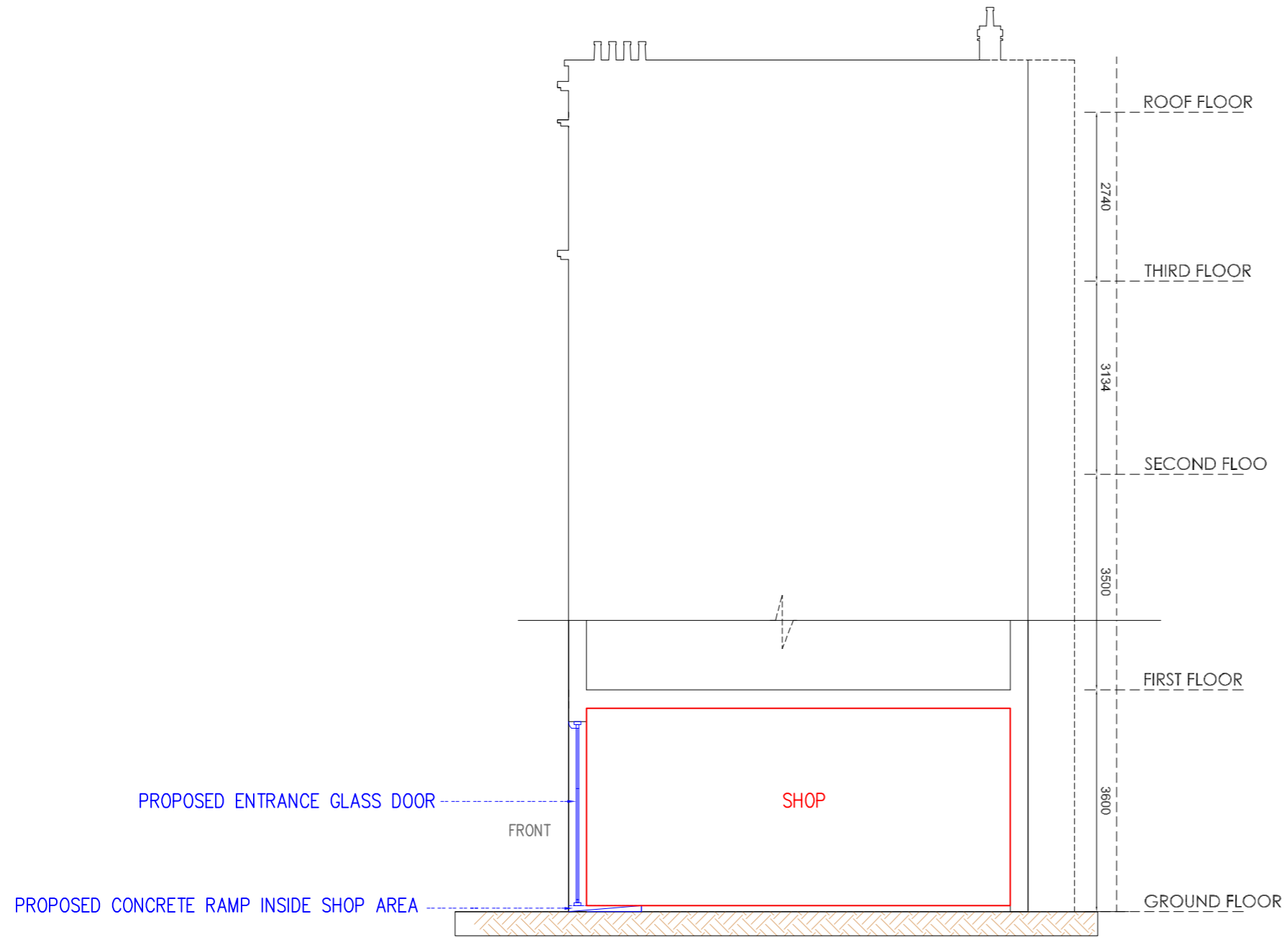
PROPOSED SECTION A-A Scale: 1:100
