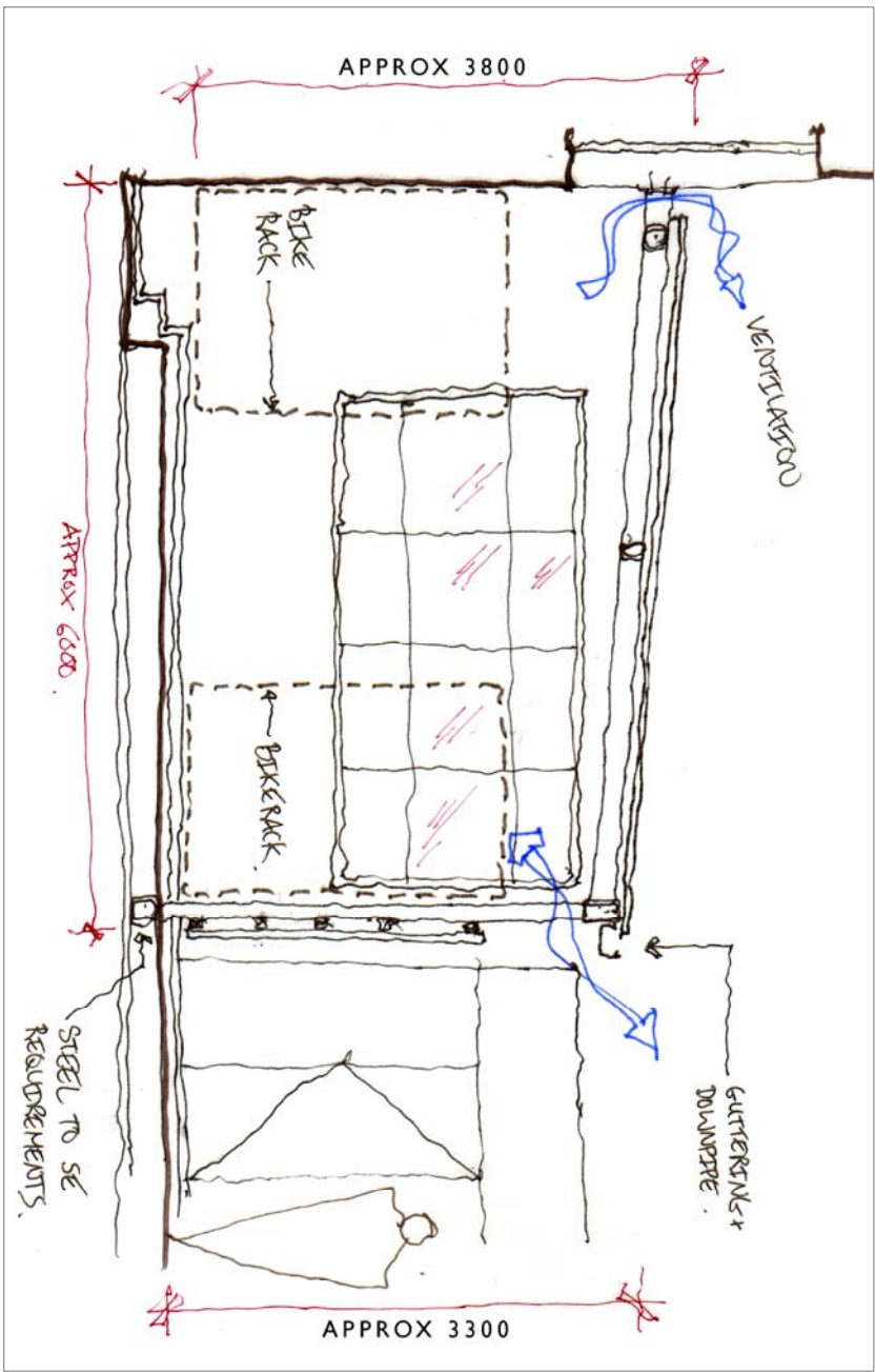
PROPOSED PLAN OF BIKE SHELTER NTS
