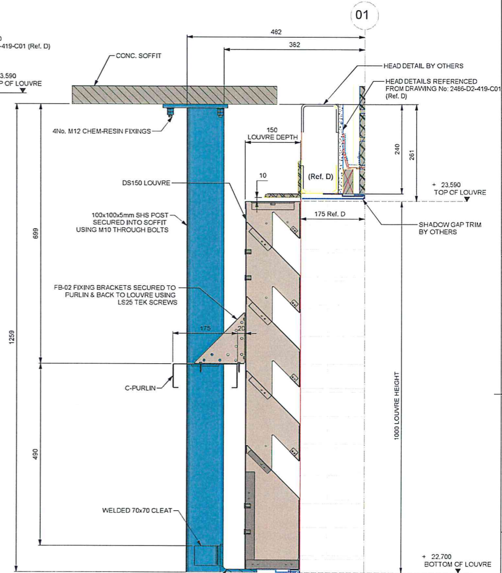
SECTIONAL VIEW: B-B DS150 CANTELOURED LOUVRE N.T.S
