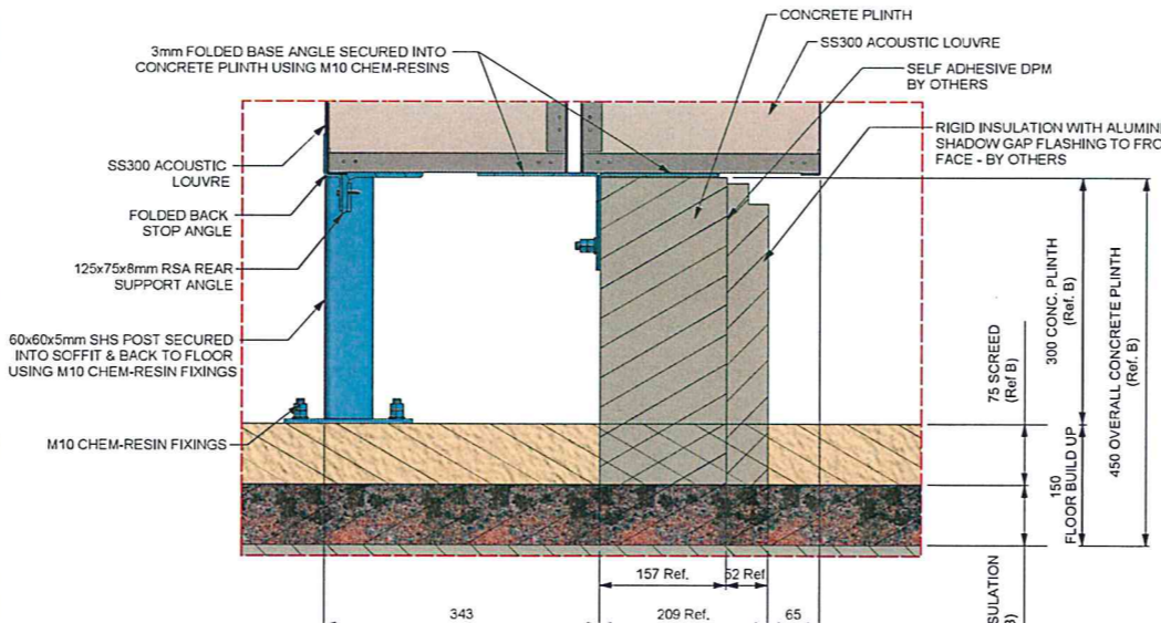
DETAIL VIEW: F BOTTOM - LOUVRE FIXING ARRANGEMENT SCALE: 1 : 5 @ A1
