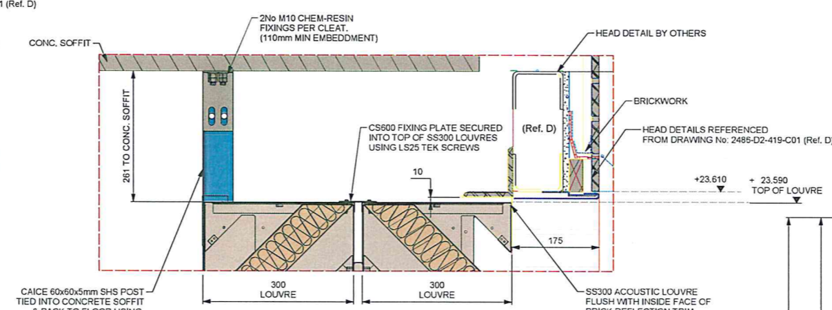
DETAIL VIEW: E TOP - LOUVRE FIXING ARRANGEMENT SCALE: 1 : 5 @ A1
