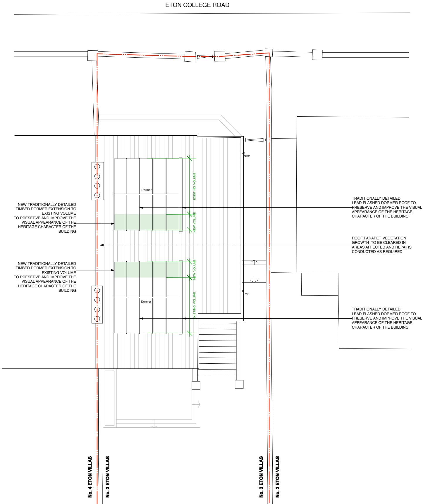
ROOF PLAN PROPOSED
