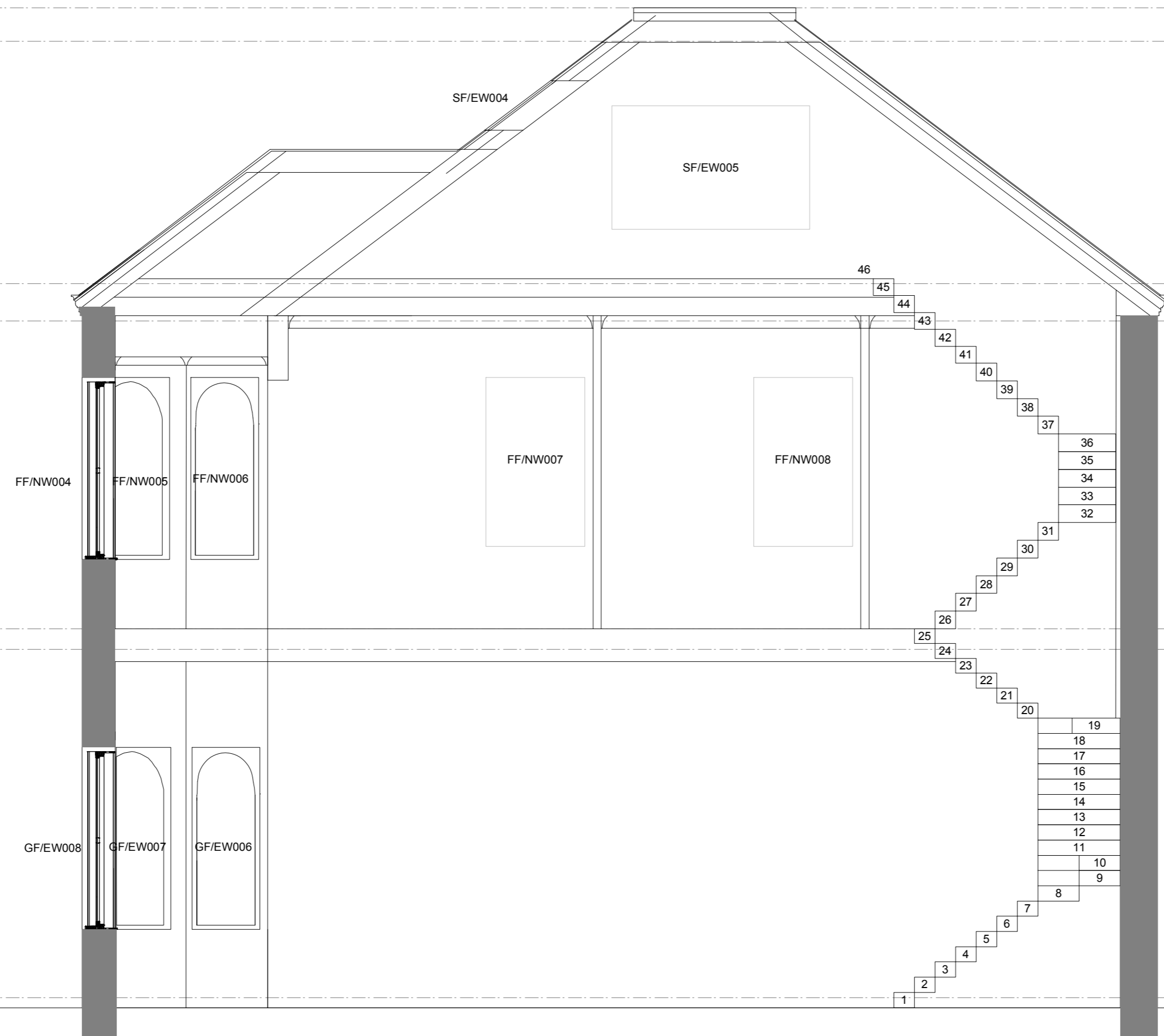
EXISTING SECTION B - B
