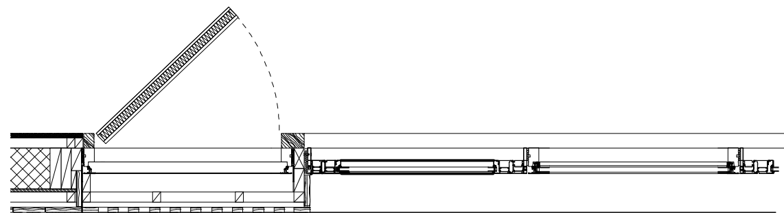
01 Enlarged Plan - Window, Cladding & Vent Interface 1:25
