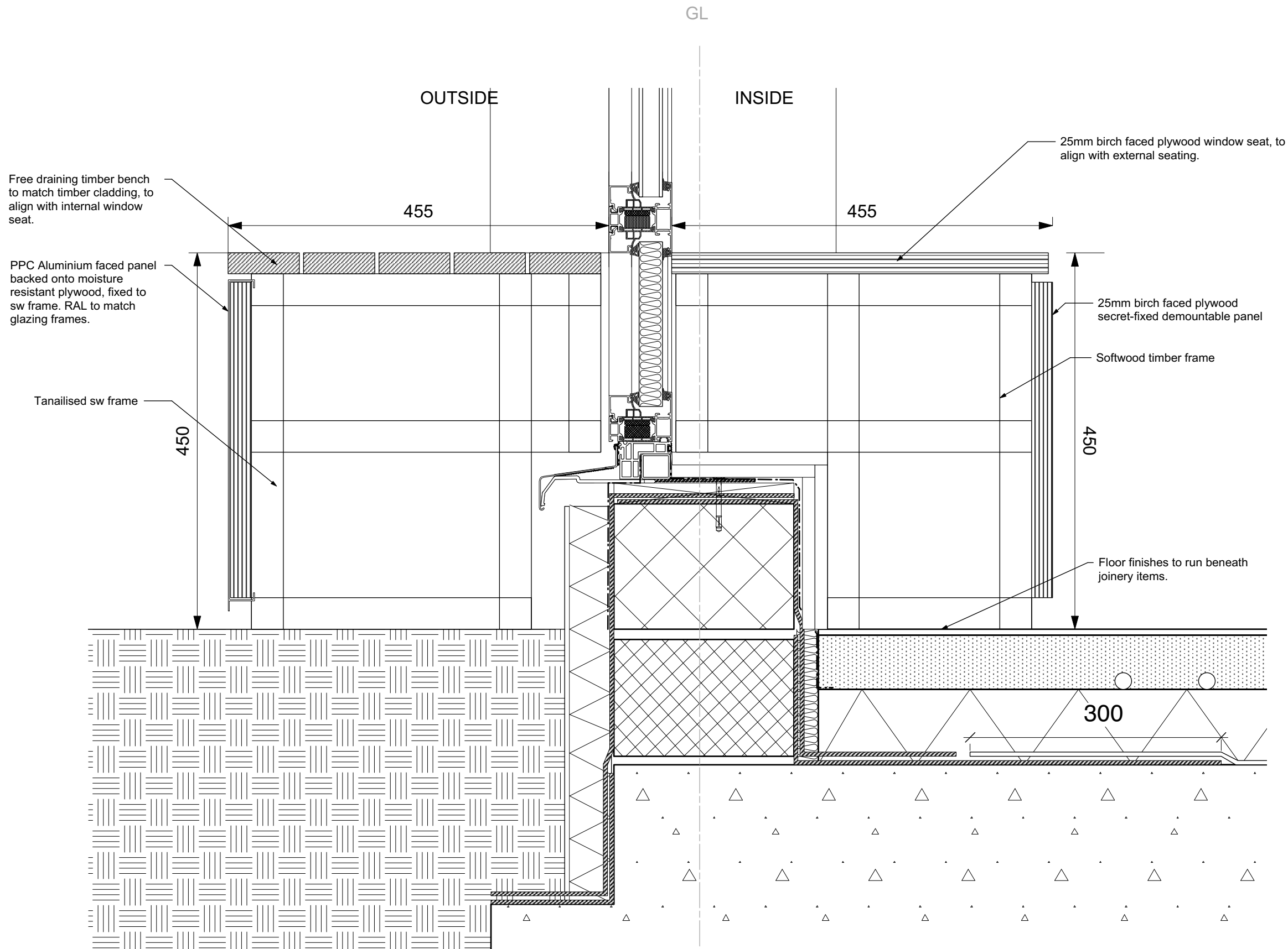
1 Cill Detail C with External Bench Seat 596_D512
