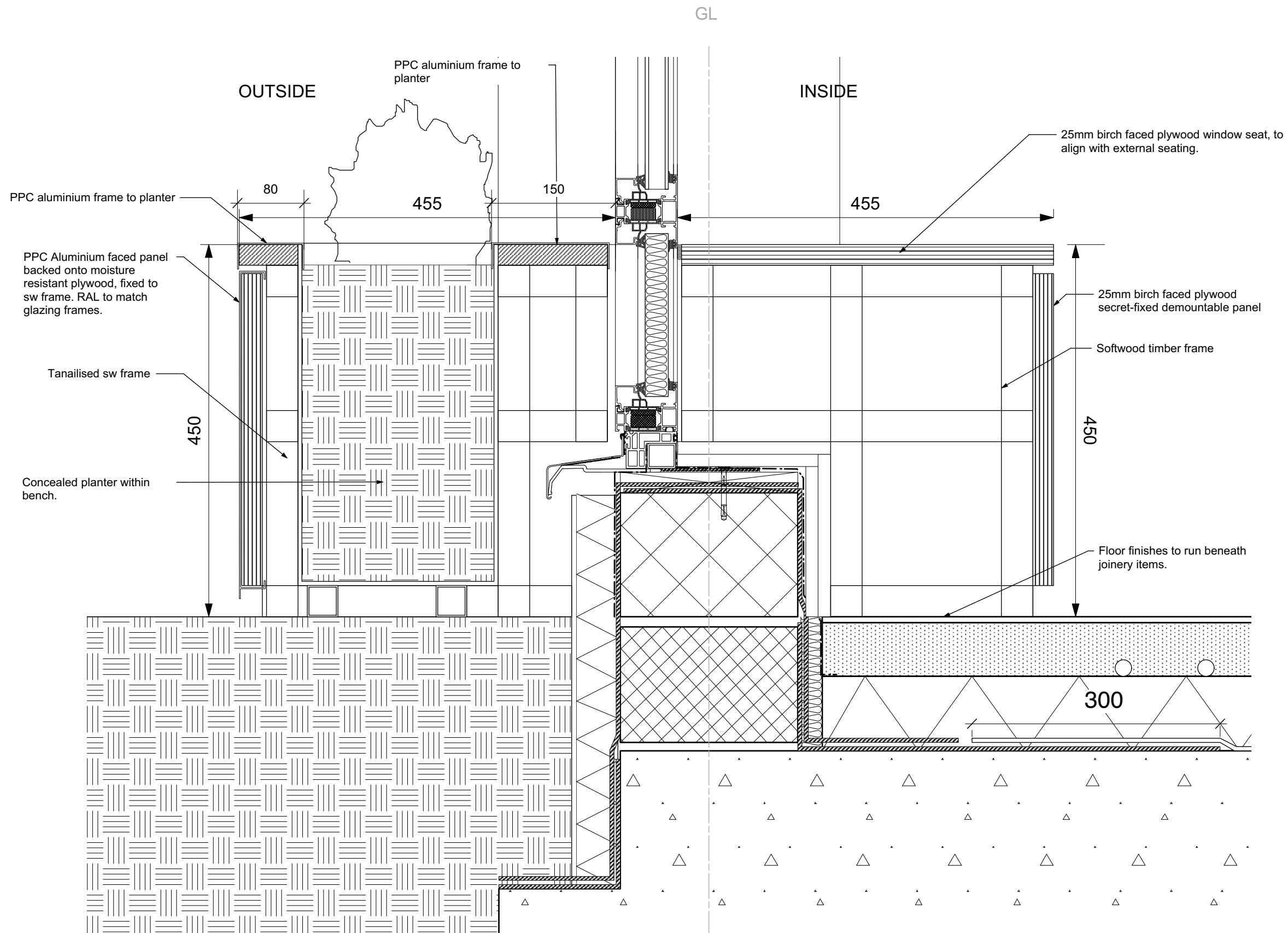
1 Cill Detail C with External Planter 596_D513
