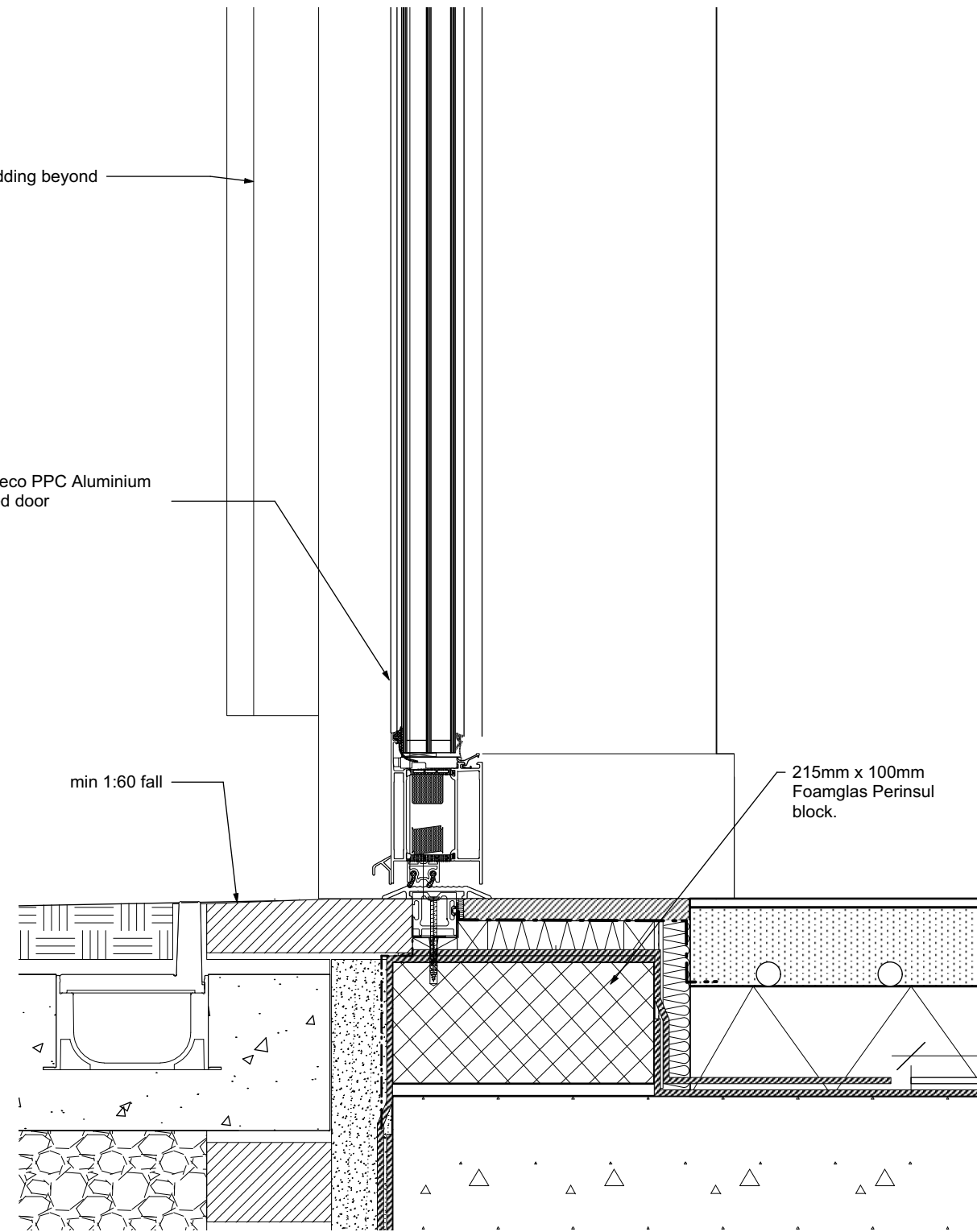
2 Threshold Detail B 596_D603
