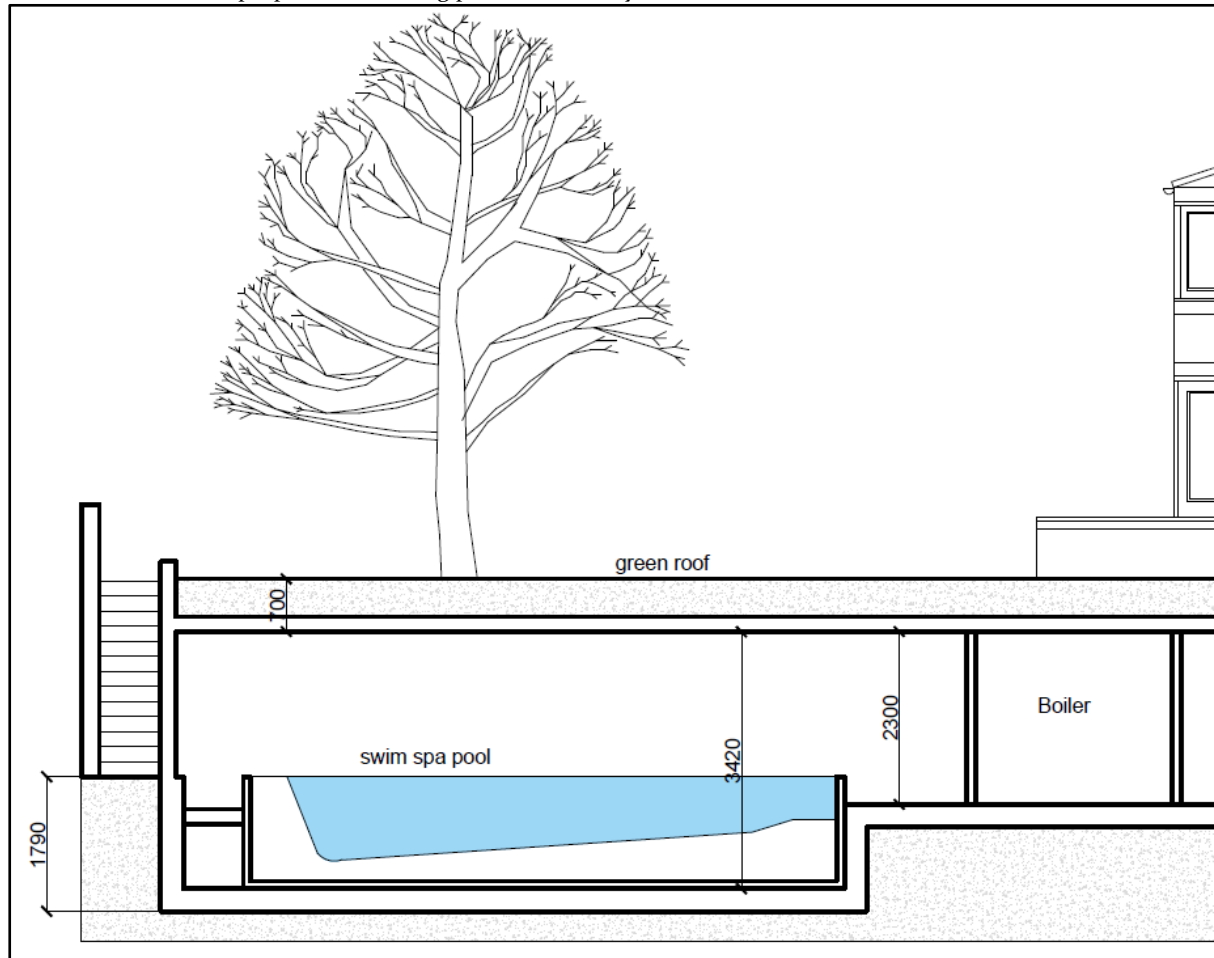
Figure 1: A section diagram showing the Oak and proposals. The nearest wall of the proposed building is 4.6m away from the Oak and the proposed swimming pool is 8.1m away.
