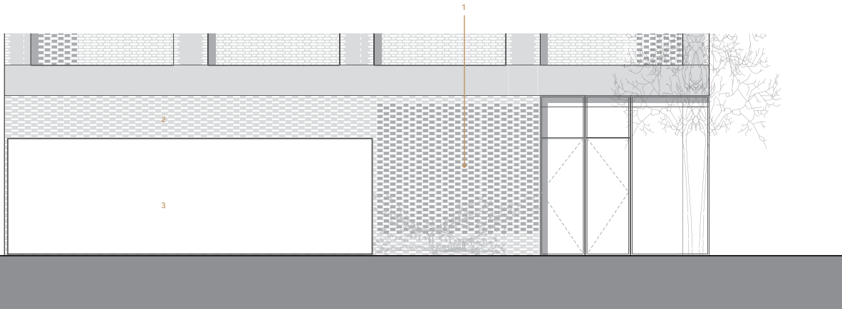
2.6 Ground floor treatment of residential entrance
