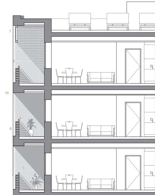
2.1 Section C-C
