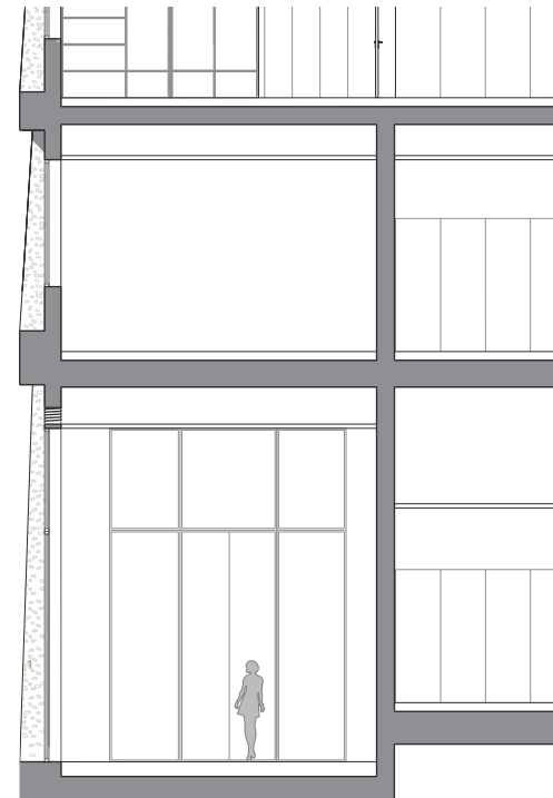
1.3 Section B-B
