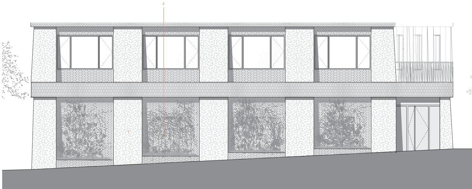
1.4 Ground floor treatment of wall flanking car park ramp - Elevation
