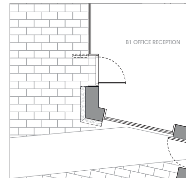
1.8 B1 office entrance corner plan
