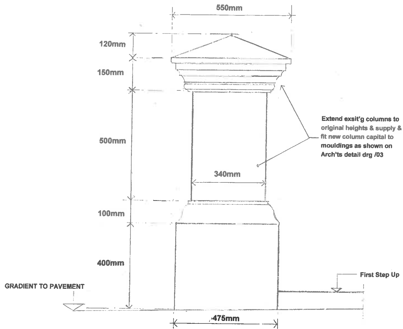
7 NEW COLUMNS & CAPITALS AS ORIGINAL DETAIL
