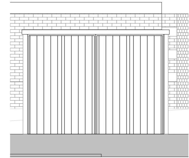
E-13 Bike Store Front Elevation 1:50
