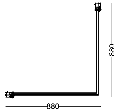
PLAN VIEW 1:20
