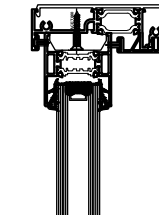
DETAIL F
