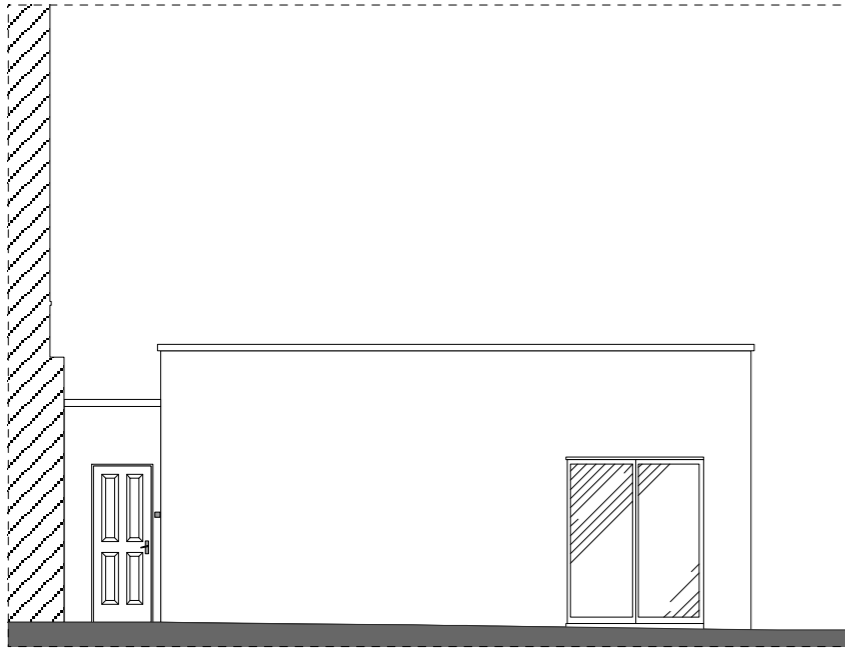
South-West Elevation
