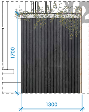
Bike Shed Side Elevation
