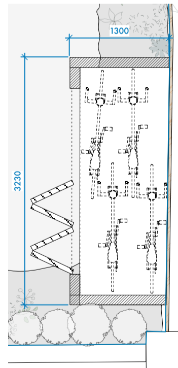
Bike Shed Plan
