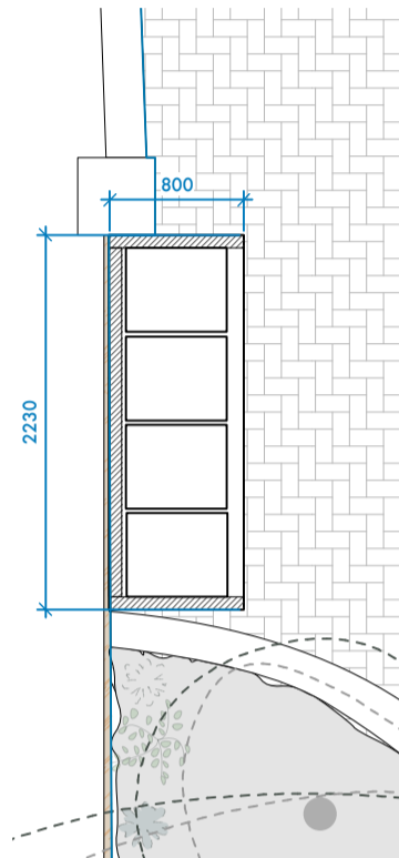
Bin Store Plan
