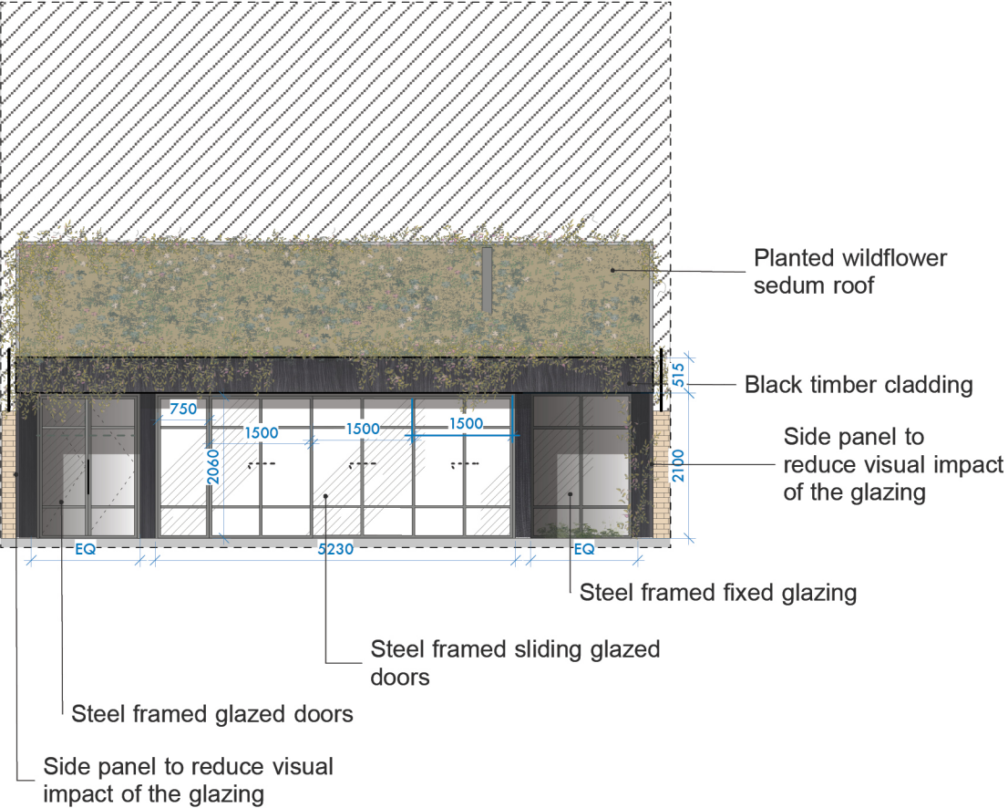
Front Elevation
