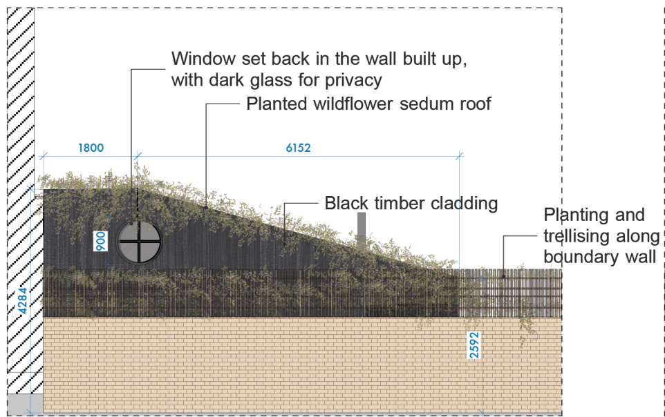
South-West Elevation
