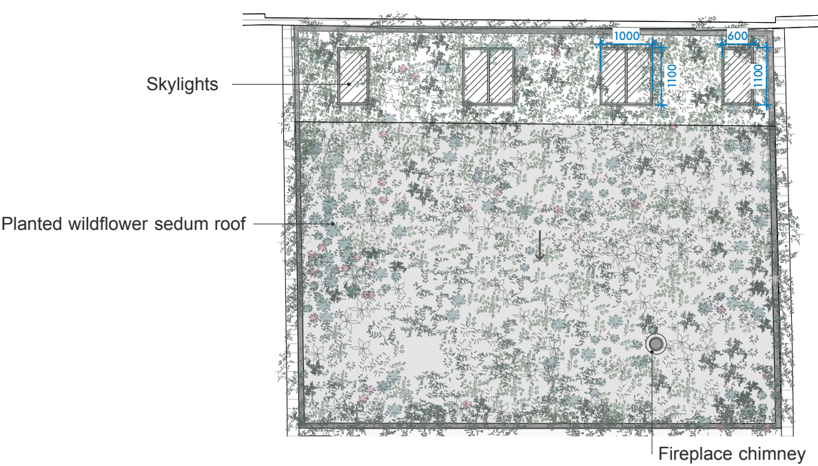
Roof Plan
