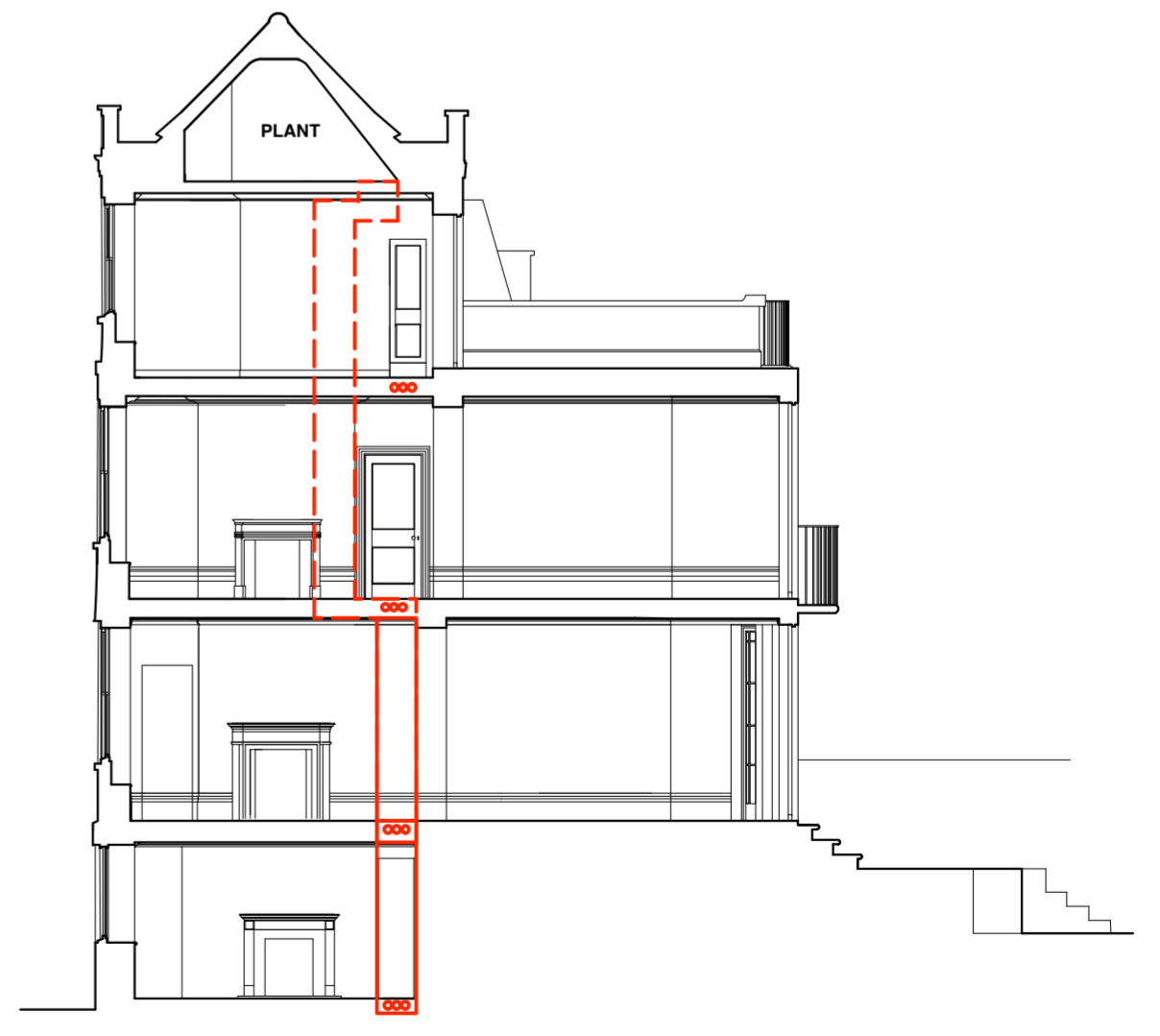
SECTION YY 1:100
