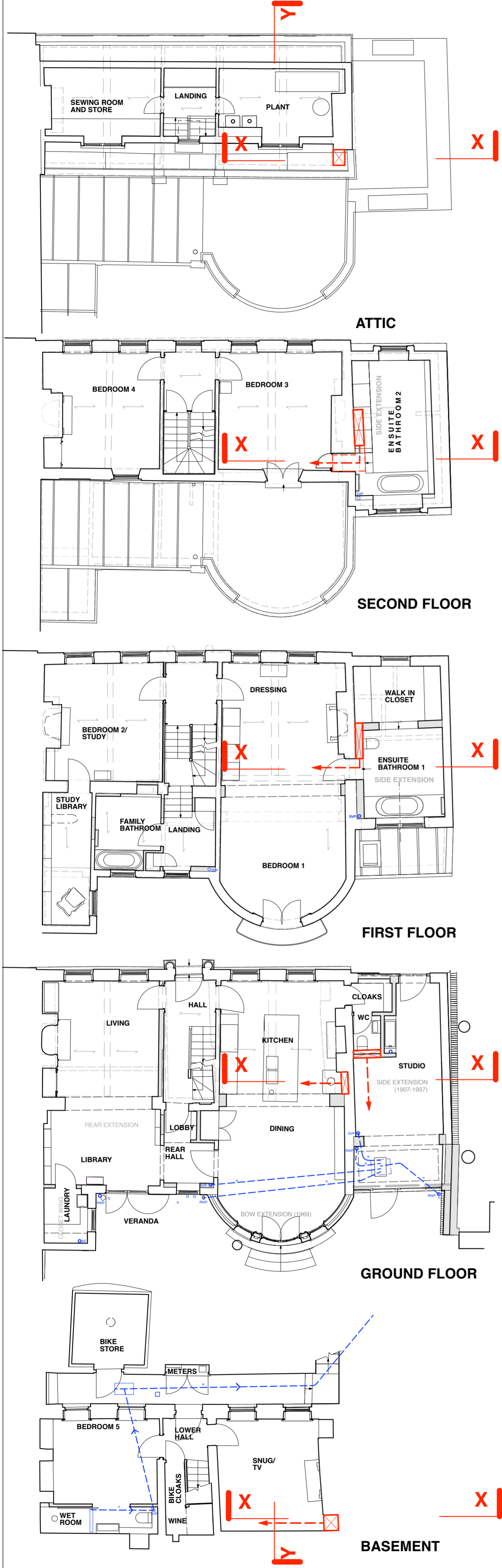
PLANS 1:100
