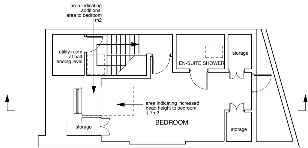
Proposed 4th Floor Plan 1:100 @ A3
