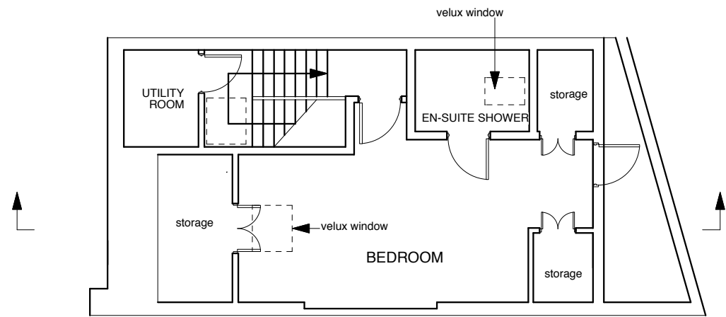
Existing 4th Floor Plan 1:100 @ A3
