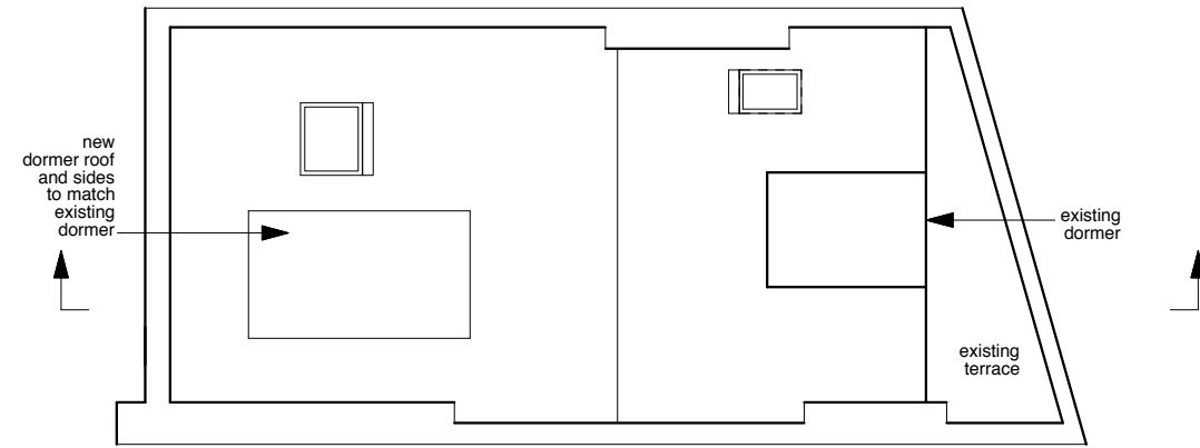
Proposed Roof Plan 1:100 @ A3
