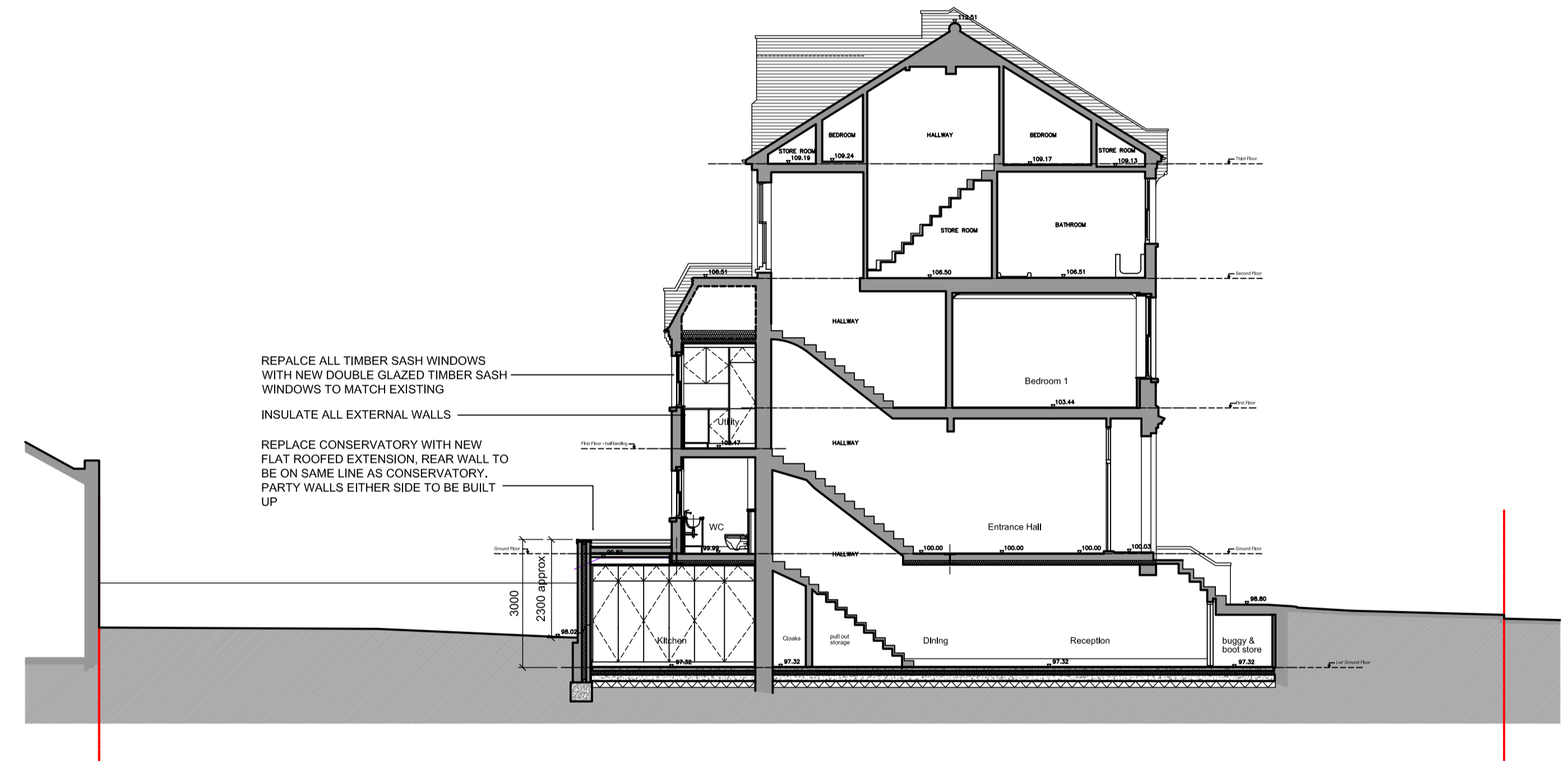
Section B-B
