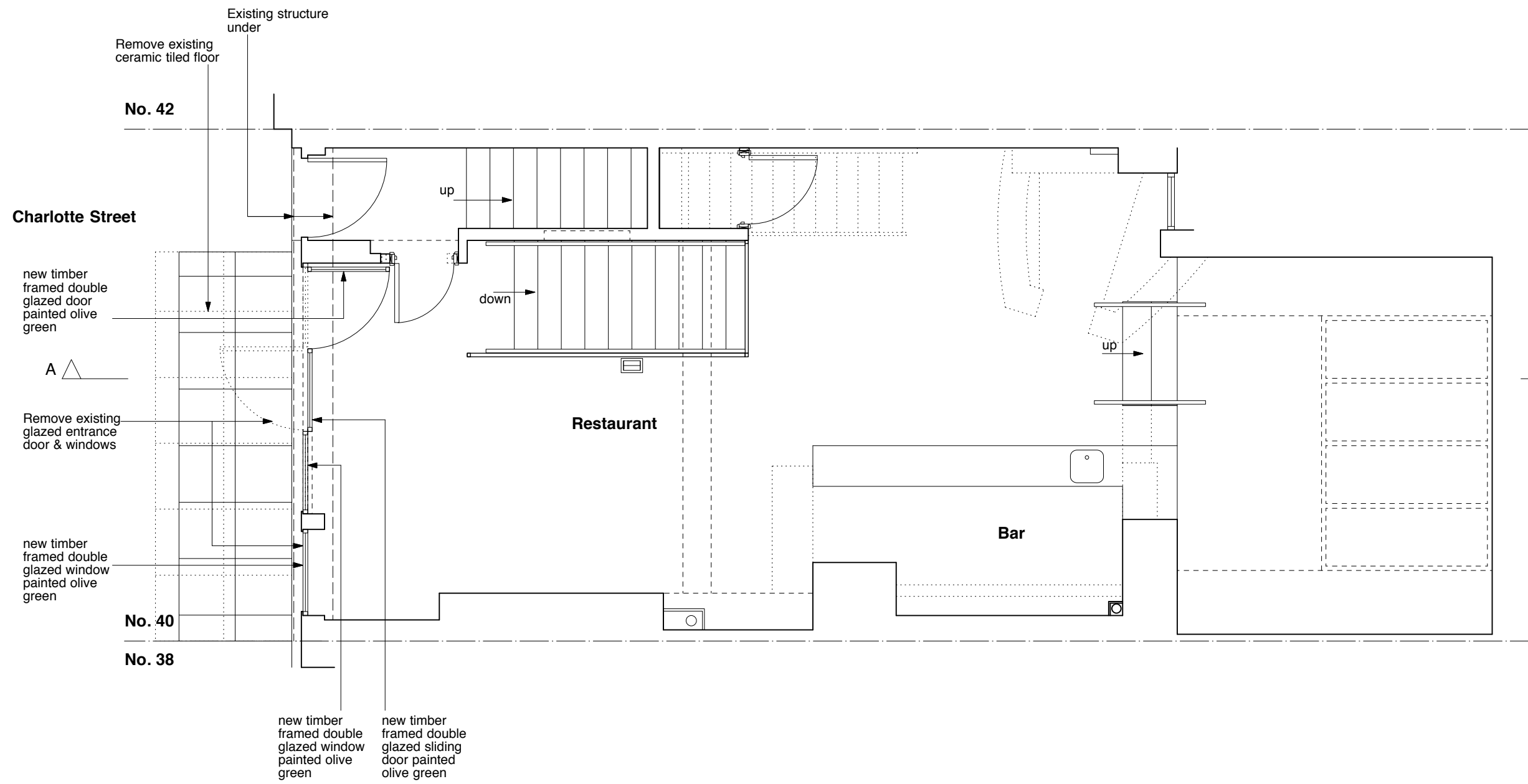
PROPOSED GROUND FLOOR PLAN scale 1:50 0 1 2 3 M
