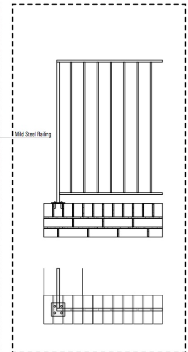
Balustrade Detail
