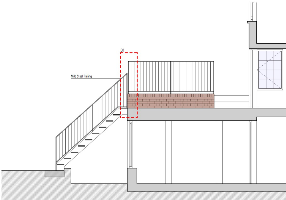
Long Section 1/50
