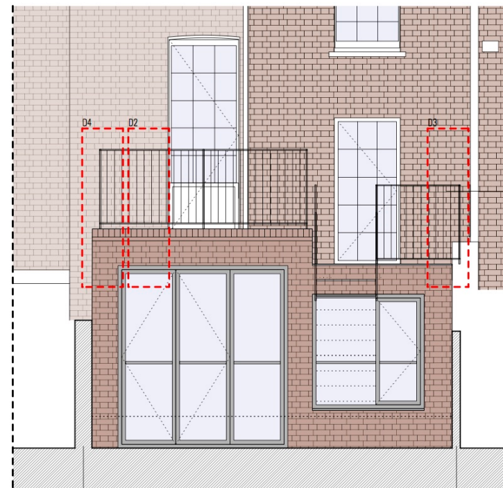
Rear Elevation 1/50
