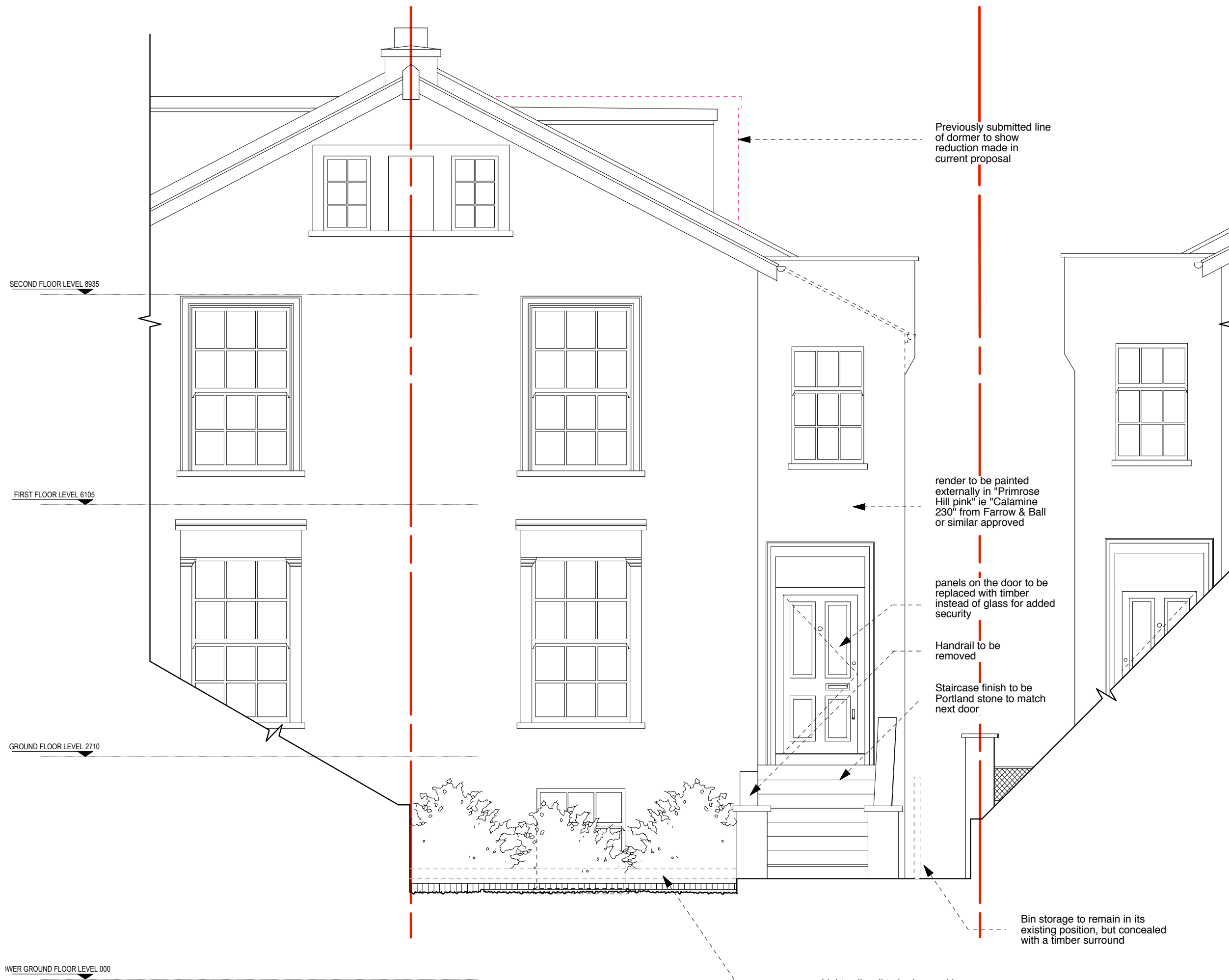
AS PROPOSED _ Front Elevation
