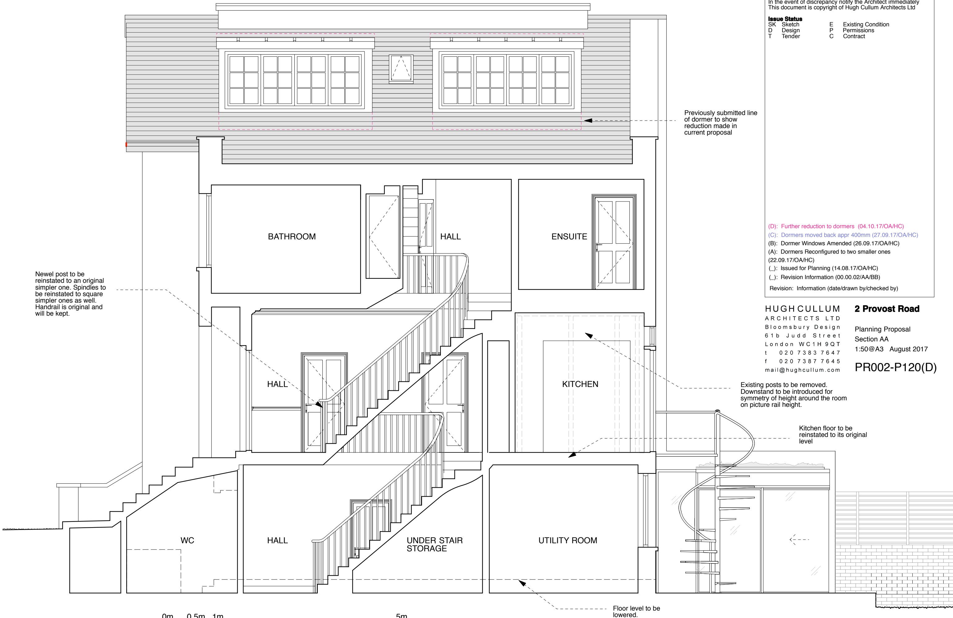
AS PROPOSED _ Section AA
