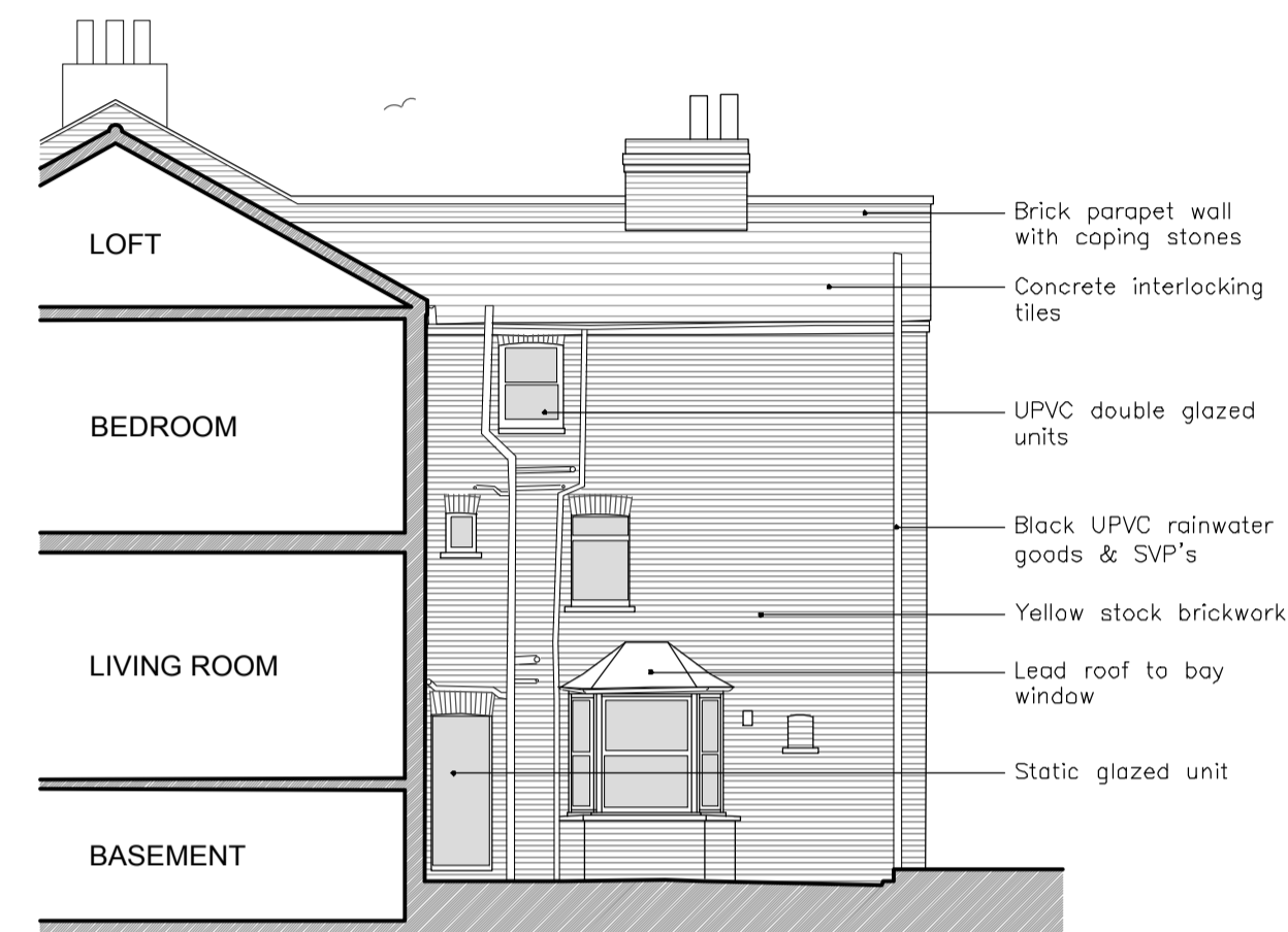
SIDE ELEVATION
