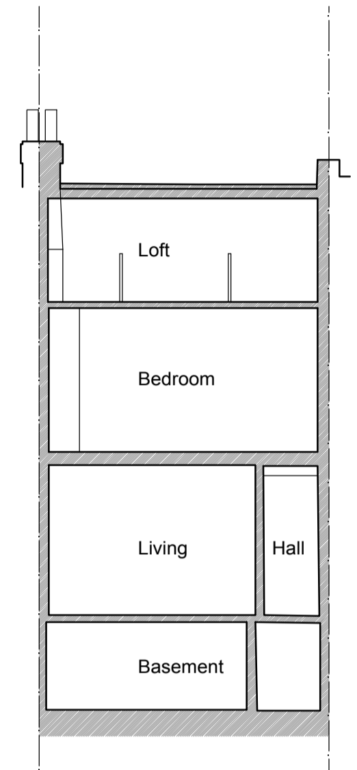
SECTION BB
