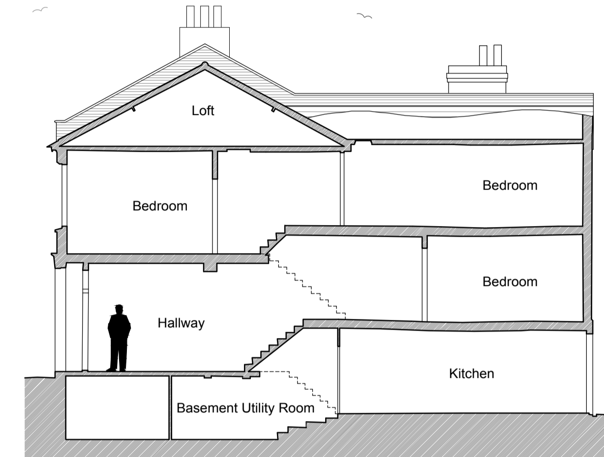
SECTION AA 1:100@A1
