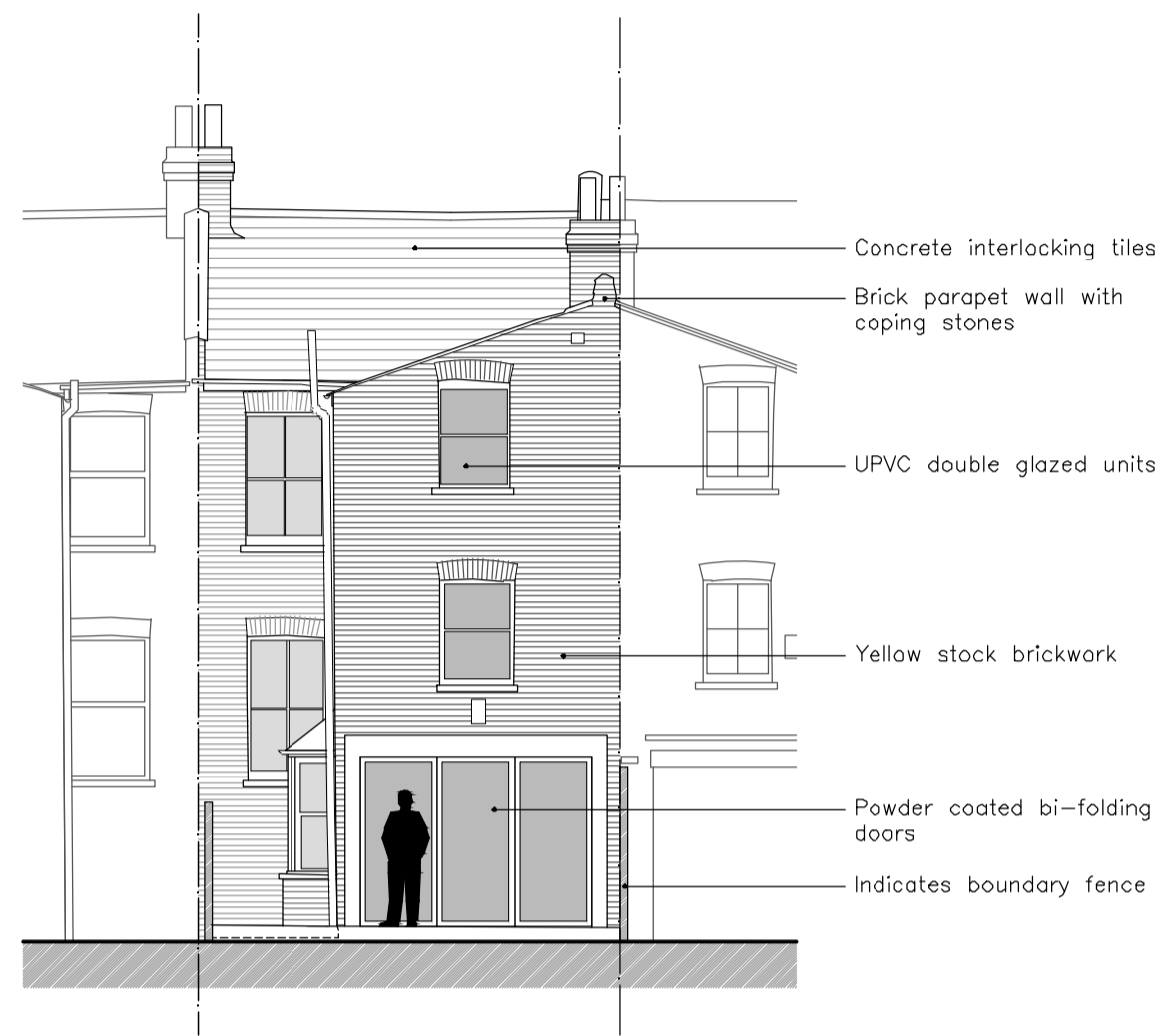
REAR ELEVATION
