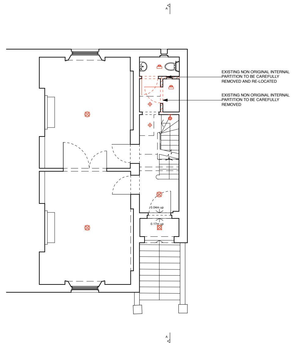
UPPER GROUND FLOOR PLAN EXISTING (RAISED GROUND) ENABLING WORKS
