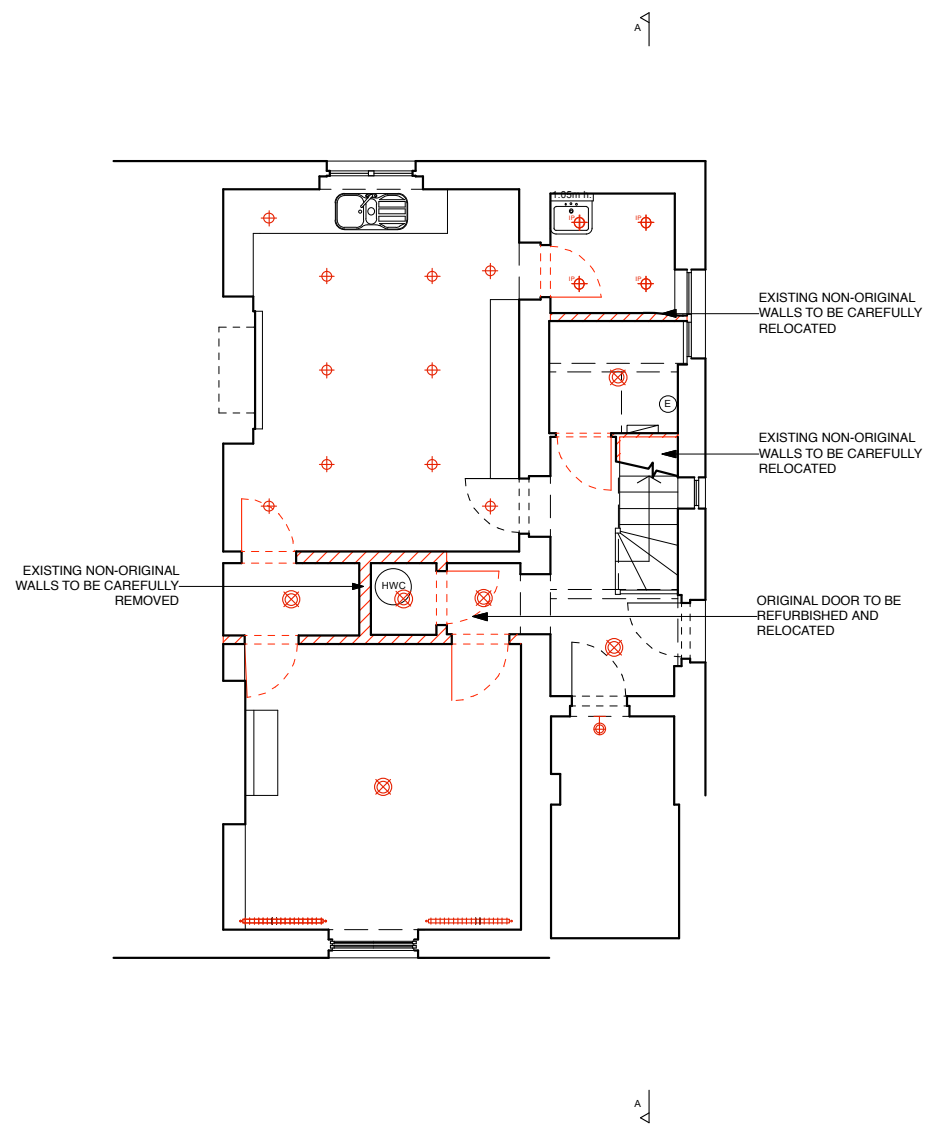
LOWER GROUND PLAN EXISTING (BASEMENT) ENABLING WORKS
