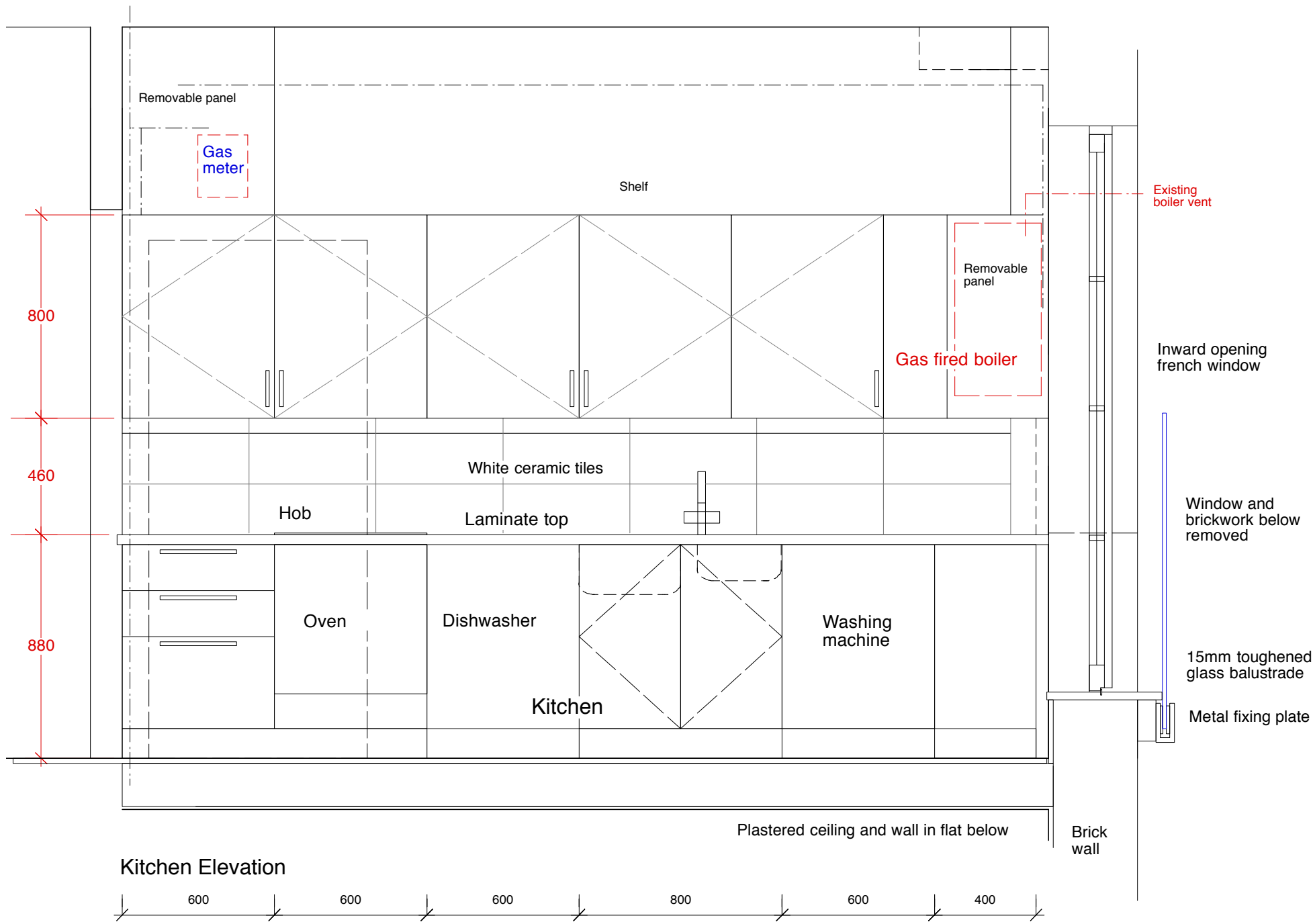
Kitchen Elevation
