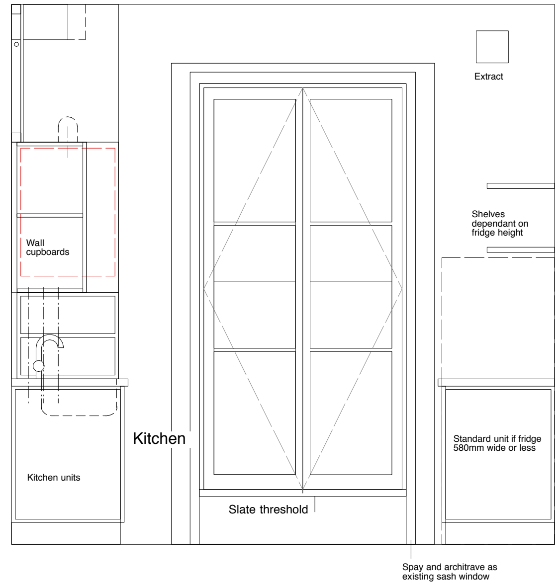
Kitchen Elevation
