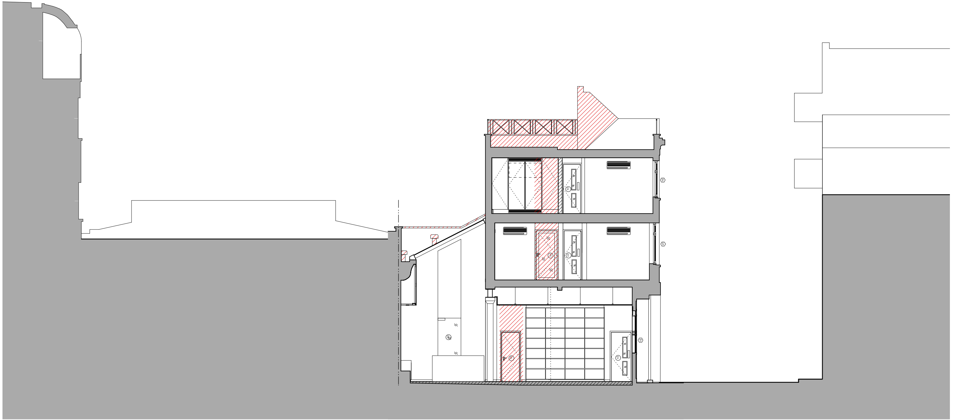
SECTION B
