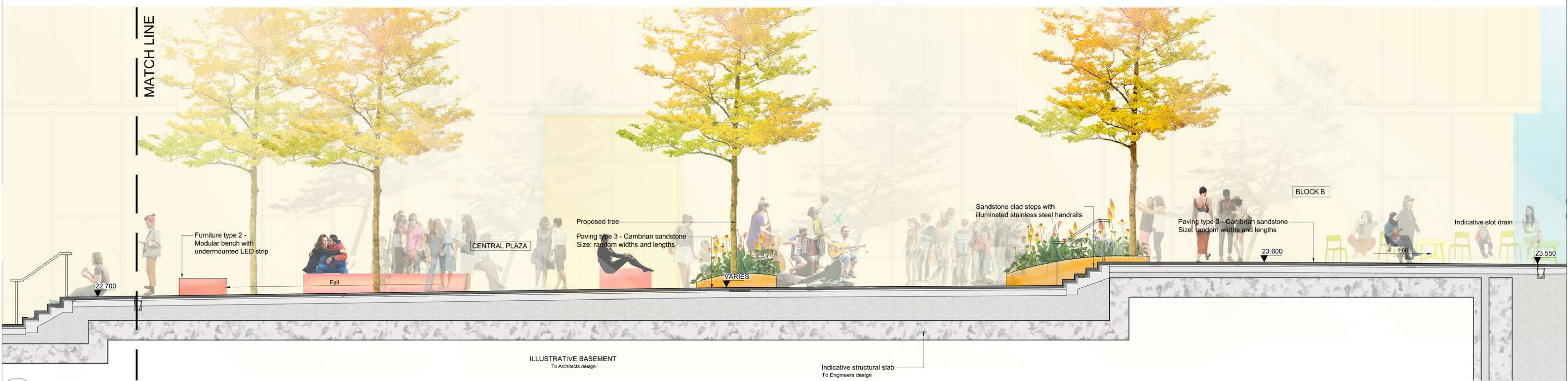
01 Landscape Section AA Through Plaza SCALE 1:50@A1
