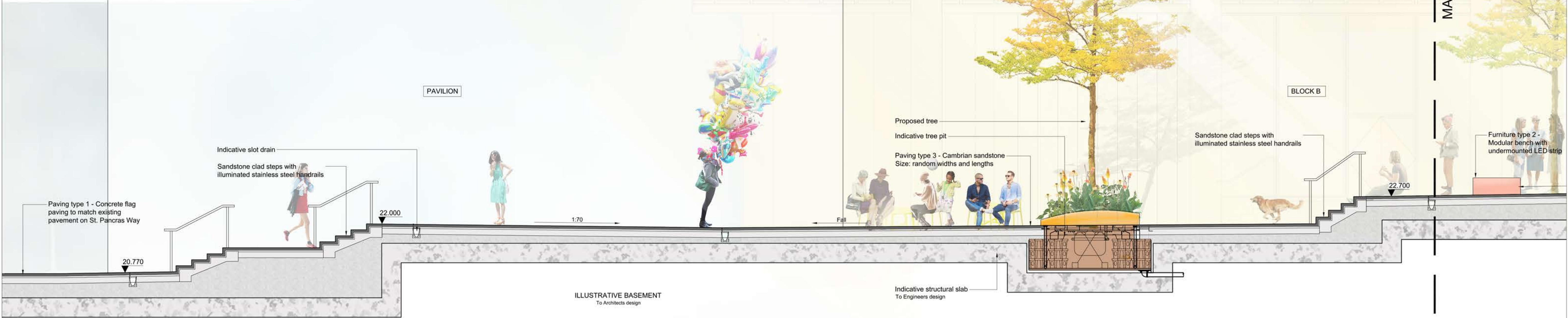
01 Landscape Section AA Through Plaza SCALE 1:50@A1
