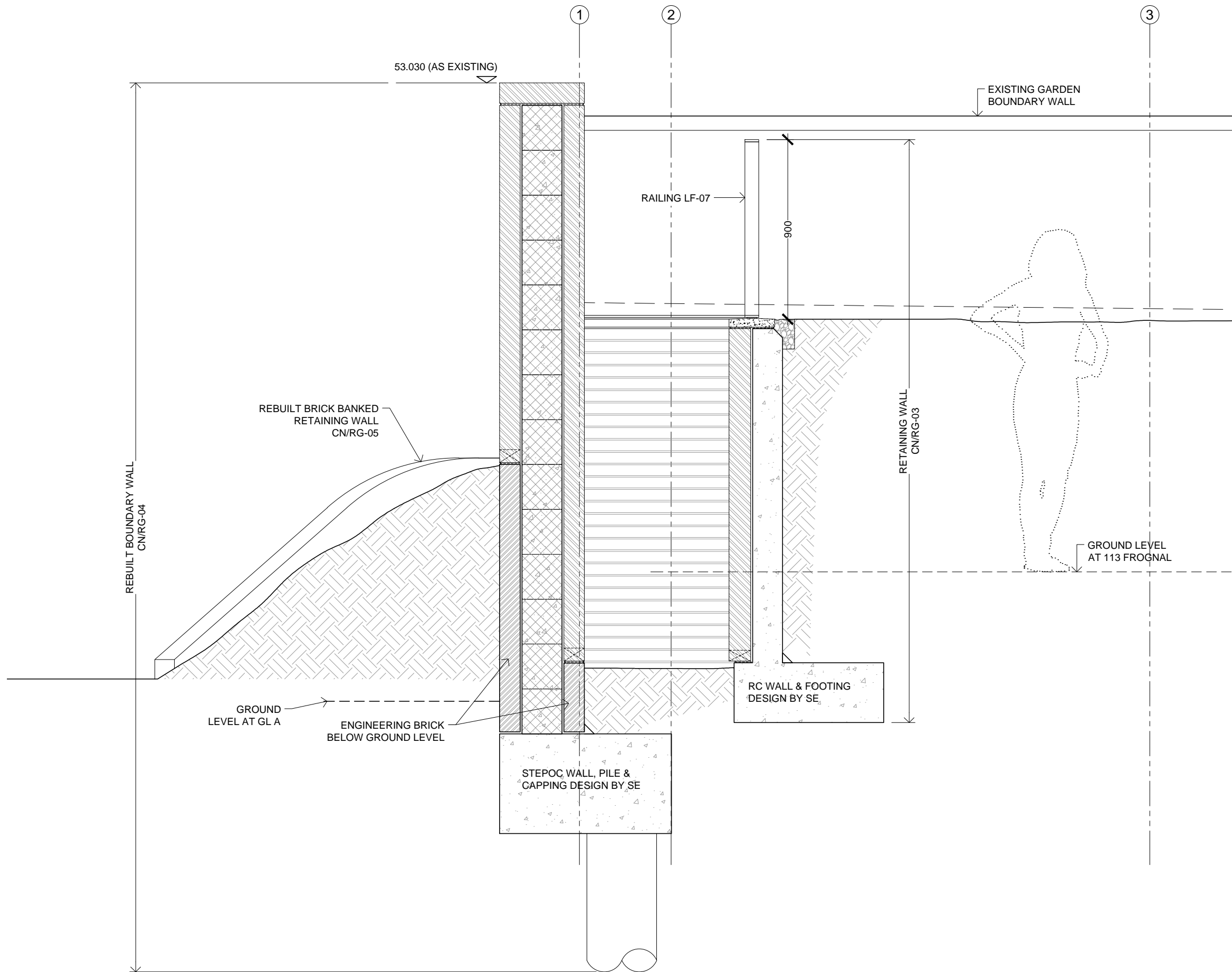
SECTIONAL DETAIL 1 1:20 @ A3 FRG-911
