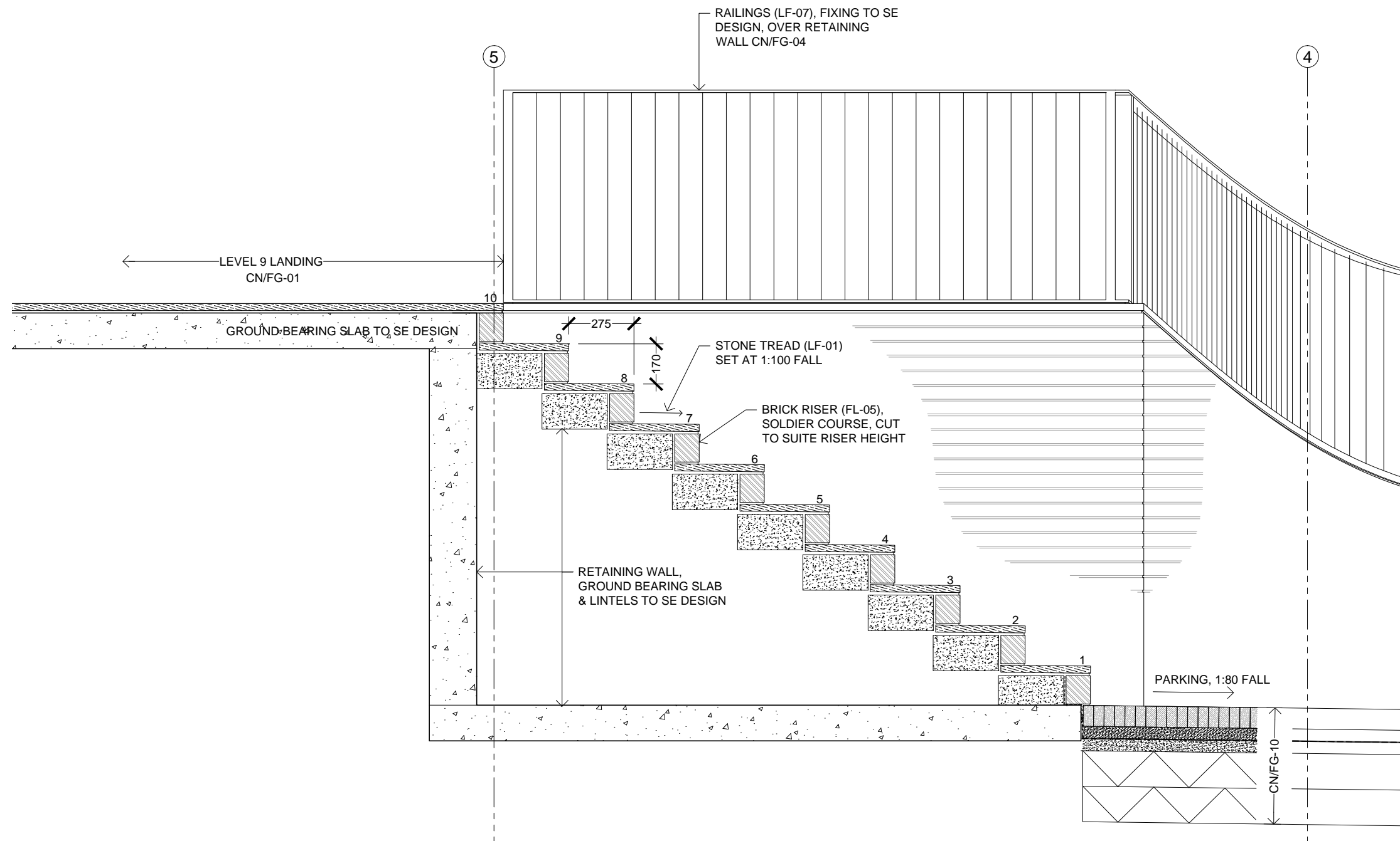
SECTION / ELEVATION 1 1:20 @ A3 FRG-910
